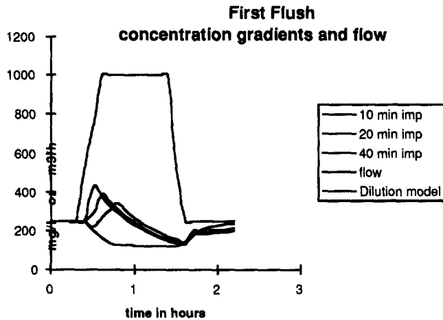
Figure 5. Simulated concentrations with 120 minutes dry weather flow as holding volume of the sewer system.
