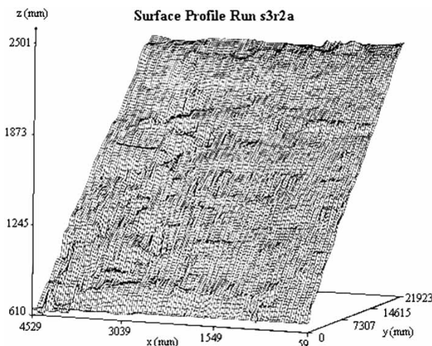
Figure 1 | Microtopographic surface of experimental plot S3R2A (Tayfur & Singh 2004).
