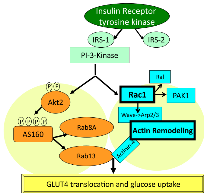
FIG. 1. Rac1 is an obligatory element in insulin signaling in muscle, leading to glucose uptake. In cultured muscle cells, insulin activates Rac1 leading to cortical actin filament remodeling, and this module is required for GLUT4 translocation, in parallel to input by the Akt2 module. Sylow et al. (8) show that Rac1 is similarly required for insulin-stimulated glucose uptake in skeletal muscle and that Rac1 or PAK1 defects are associated with insulin-resistant states in mice and humans.
