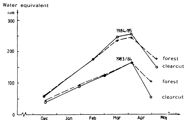
Fig. 2. Water equivalent of snow on clearcuts and in surrounding forests, part of NW Härjedalen, winters 1983-84 and 1984-85. Difference in snow pack between the clearcuts was considerable at the end of April.
