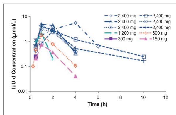
Figure 1. Plasma exposures of the active metabolite IdUrd following a single dose of IPdR over the range of 150 to 2,400 mg. Plasma concentrations remained above 1 \mu\text{mol/L} for 3 to 4 hours and declined with a half-life of 1.5 hours.
