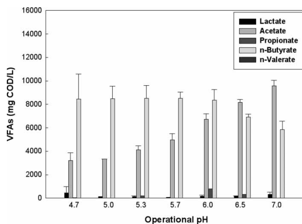
Figure 4 | The effect of operational pH values on VFA production during dark H 2 fermentation of food waste.
