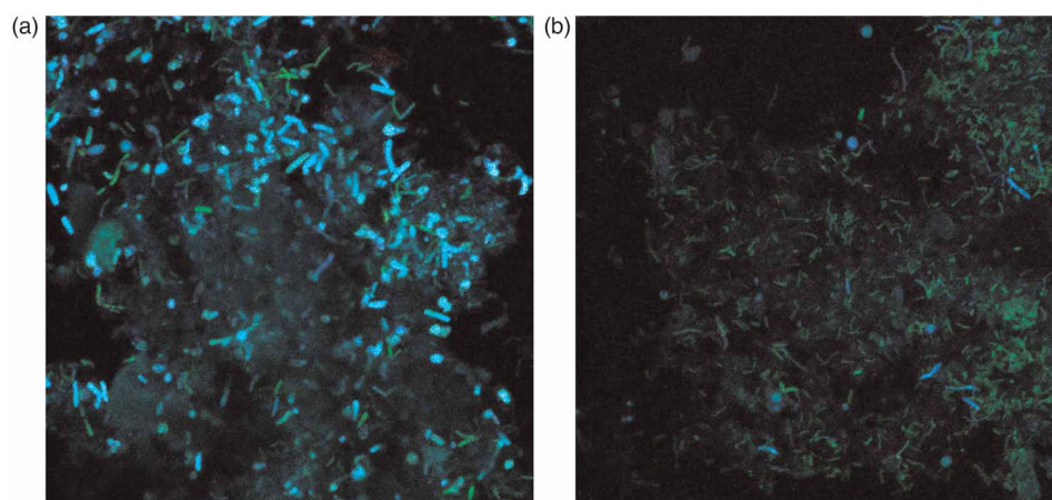
Figure 5 | FISH analysis of microorganisms at operational pH 5.3 (a) and 7.0 (b). Eubacteria were detected by FAM-labeled EUB338 (green), Clostridium species of Cluster I and XI were detected by Cy5-labeled P932 (blue), and Clostridium species of Cluster I and II were detected by Cy3-labeled Chis 150 (red).
