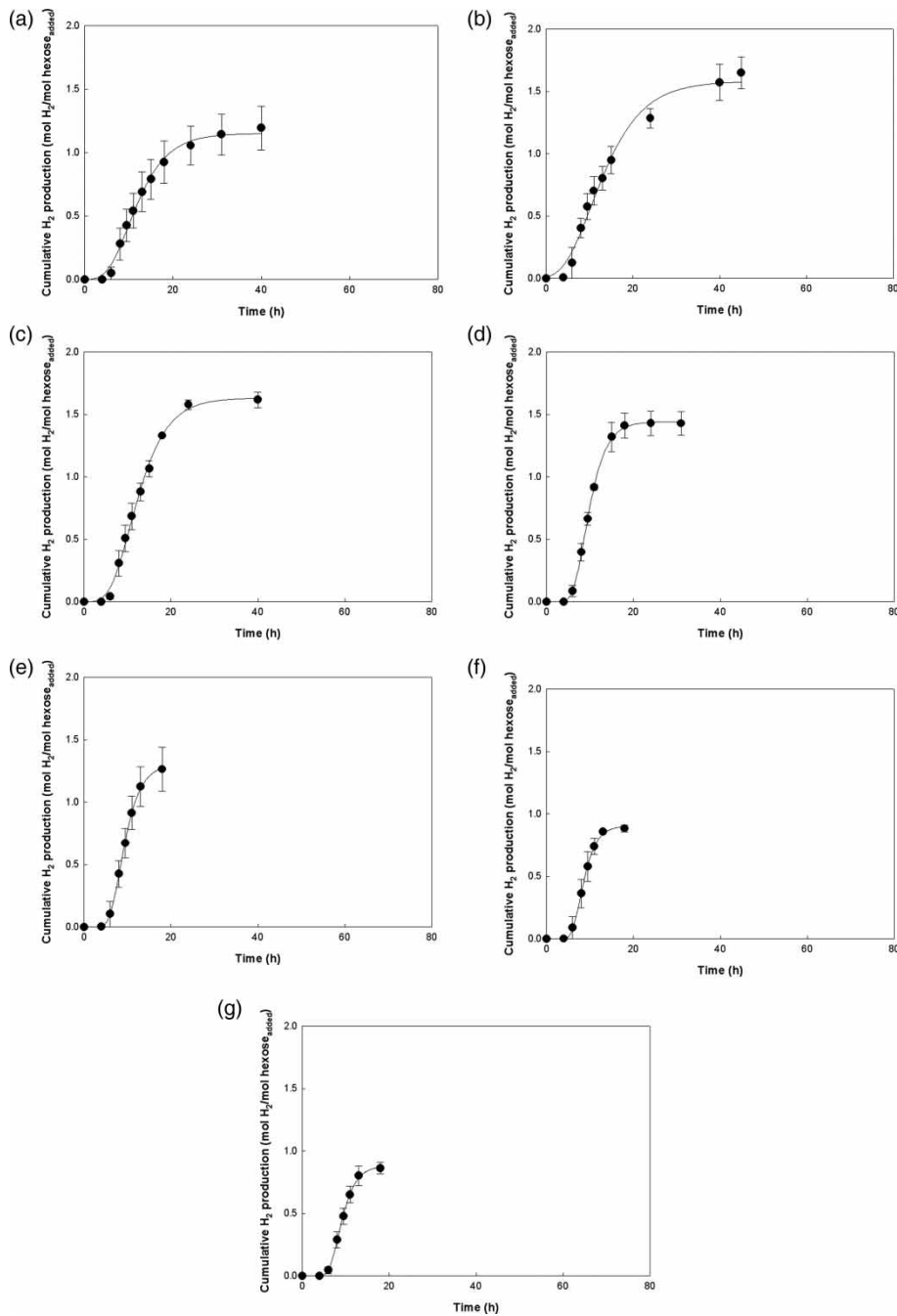
Figure 2 | The effect of operational pH values on cumulative hydrogen production during dark H 2 fermentation of food waste. (a) pH 4.7, (b) pH 5.0, (c) pH 5.3, (d) pH 5.7, (e) pH 6.0, (f) pH 6.5, (g) pH 7.0.
