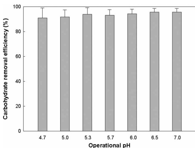
Figure 3 | The effect of operational pH values on carbohydrate removal efficiency during dark H 2 fermentation of food waste.
