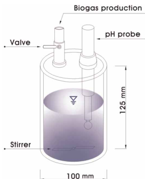
Figure 1 | Schematic diagram of anaerobic hydrogen batch reactor.
