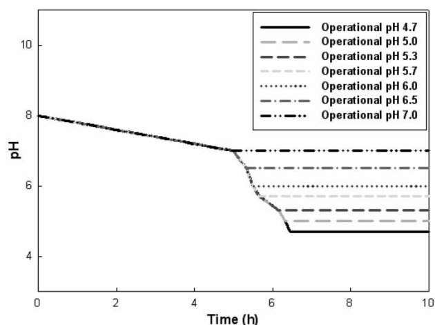
Figure 6 | pH change profile at initial stage depending on operational pH values.
