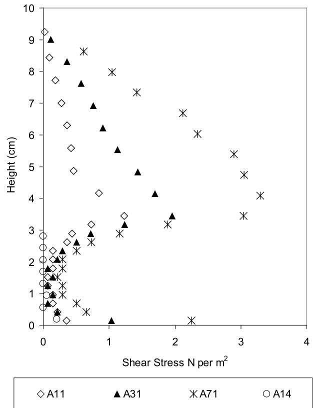
Figure 10 | Shear stress distribution obtained from method 2.
