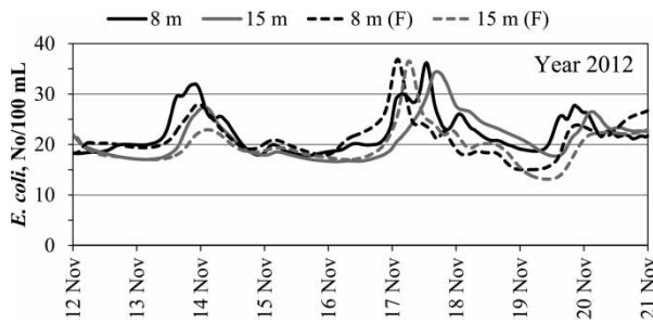
Figure 6 | Modelling results: the E. coli concentrations at the 8 and 15 m water intakes simulated using the observed input data ('8 m' and '15 m', respectively) and the forecast input data ('8 m (F)' and '15 m (F)', respectively).
