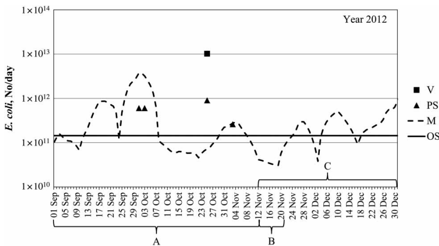
Figure 2 | E. coli load to Lake Rådasjön and simulated periods. The contamination sources are: the river Mölndalsån (M), the on-site sewage treatment systems (OS), the stream Vällbäcken (V) and the Pixbo Päls pumping station (PS). (A) and (C) represent the periods for the hindcast simulations, (B) represents the period for the forecast simulation.
