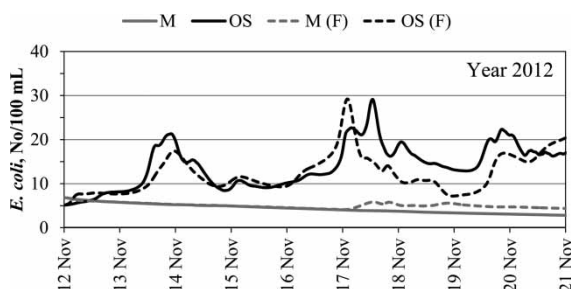
Figure 7 | Modelling results: the contributions to the E. coli concentrations at the 8 m water intake from the on-site sewage treatment systems and the river Mölndalsån simulated using the observed input data ('M' and 'OS', respectively) and the forecast data ('M (F)' and 'OS (F)', respectively).
