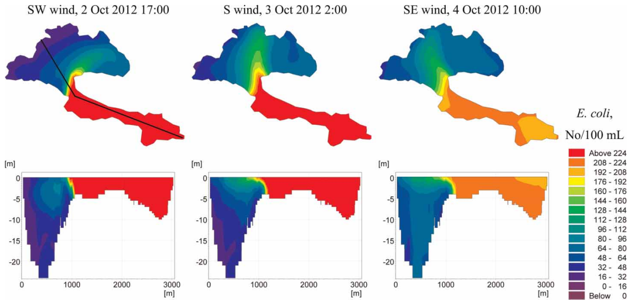
Figure 5 | Modelling results: the spread of the faecal contamination ( E. coli , No/100 mL) from the river Mölndalsån within Lake Rådasjön on 2, 3 and 4 October 2012. Top and bottom rows represent horizontal and cross-section views, respectively. The approximate location of the cross-section is shown in the top left figure.
