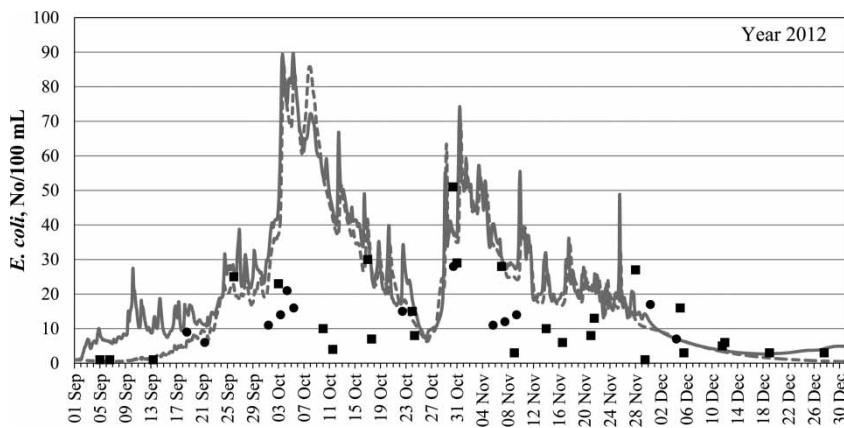
Figure 4 | Simulated (continuous and dotted lines) and measured (circles and squares) E. coli concentrations at the 8 and 15 m water intakes, respectively.
