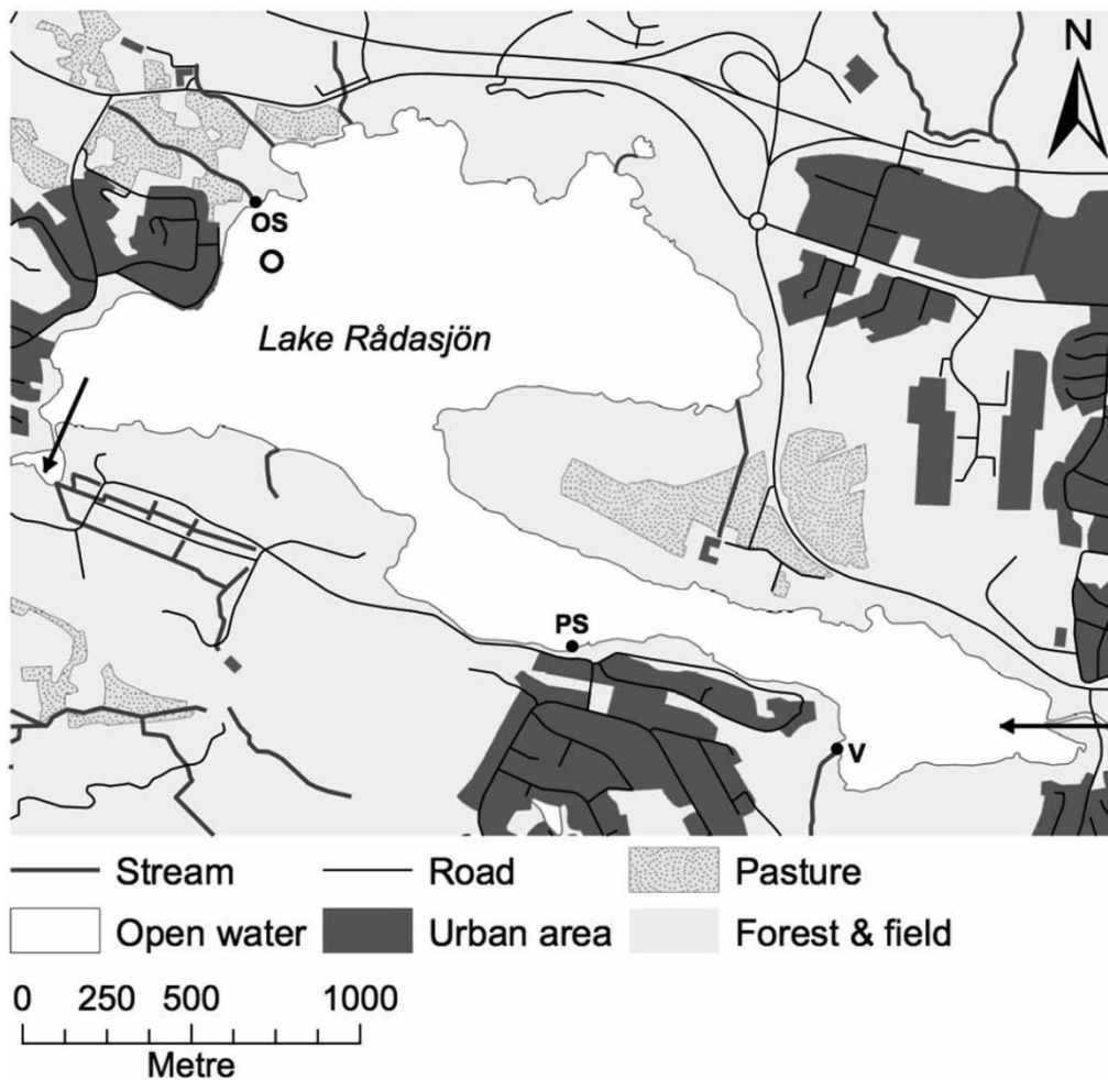
Figure 1 | Map of Lake Rådasjön. Symbols: OS – the on-site sewage treatment systems, PS – the pumping station Pixbo Päls, V – the stream Vällbäcken that transports emergency wastewater discharges. Black arrows represent the inflow to the lake from the river Mölndalsån and the outflow from the lake to Lake Stensjön. The circle represents the location of the raw water intakes.
