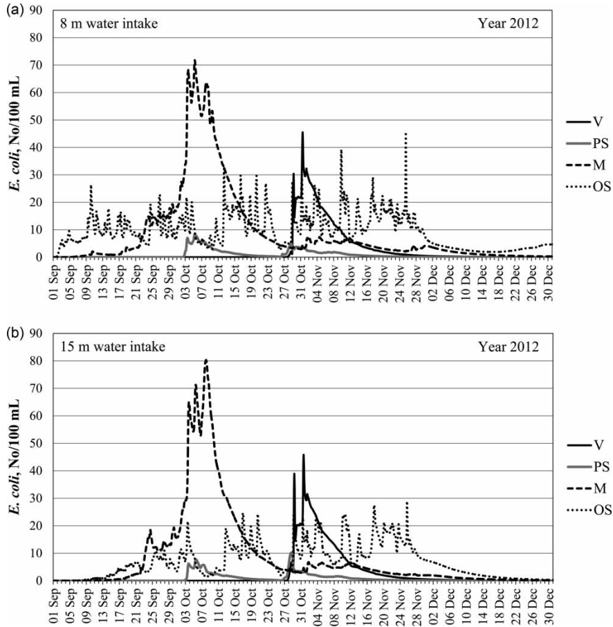
Figure 3 | Modelling results: the contribution from the different contamination sources (V – the stream Vällbäcken, PS – the pumping station Pixbo Päls, M – the river Mölndalsån, OS – the on-site sewage treatment systems) to the total E. coli concentrations at the 8 m (a) and 15 m (b) water intakes in Lake Rådasjön.
