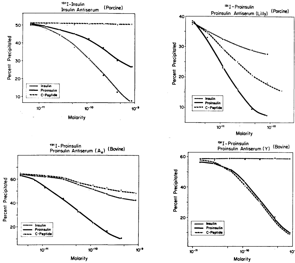
FIG. 1. Reaction of homologous insulin, proinsulin and C-peptide standards with porcine insulin (11-0) (top left), porcine proinsulin (Lilly) (top right), bovine proinsulin (A 6 ) (bottom left) and purified bovine proinsulin (Y) (bottom right) antisera. The ordinate indicates the percentage counts in the precipitate (antibody bound) after addition of the rabbit antinegative pig globulin serum.
