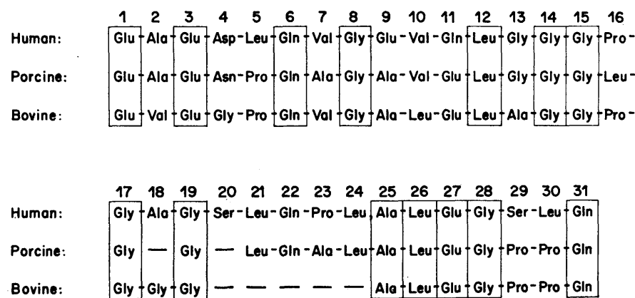
FIG. 7. Comparison of the amino acid sequences of human, 13 porcine 5 and bovine 7 C-peptides. Arbitrary deletions in the porcine and bovine molecules have been assumed to enable the best comparisons to be made. The numbers refer to the amino acid positions in bovine proinsulin. The amino acids which are identical in all three C-peptides have been enclosed in boxes.
