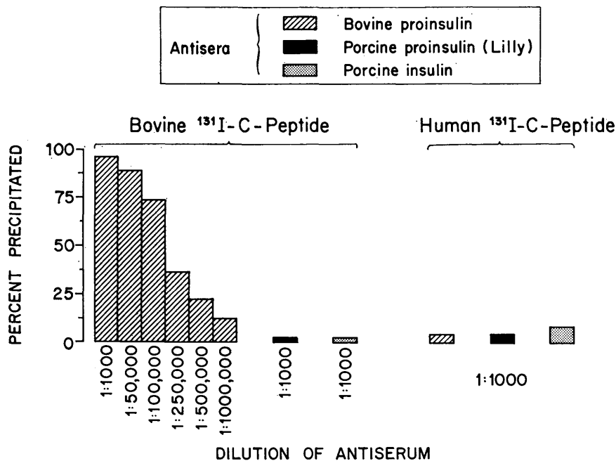
FIG. 3. Incubation of bovine (0.5 \mu g.) and human (0.5 \mu g.) I- 131 -tyrosylated C-peptide with bovine proinsulin ( A_6 ), porcine proinsulin (Lilly) and porcine insulin (11-0) antisera. The antisera were added to 1.0 ml. buffer to give final dilutions of 1:1,000 to 1:1,000,000 (bovine proinsulin antiserum), and 1:1,000 (porcine proinsulin and porcine insulin antisera). After seventy-two hours' incubation, the free and bound tracer was separated by the addition of rabbit anti-guinea pig globulin serum and the percentage bound (on the ordinate) was calculated by counting both the precipitate and supernatant after centrifugation.
