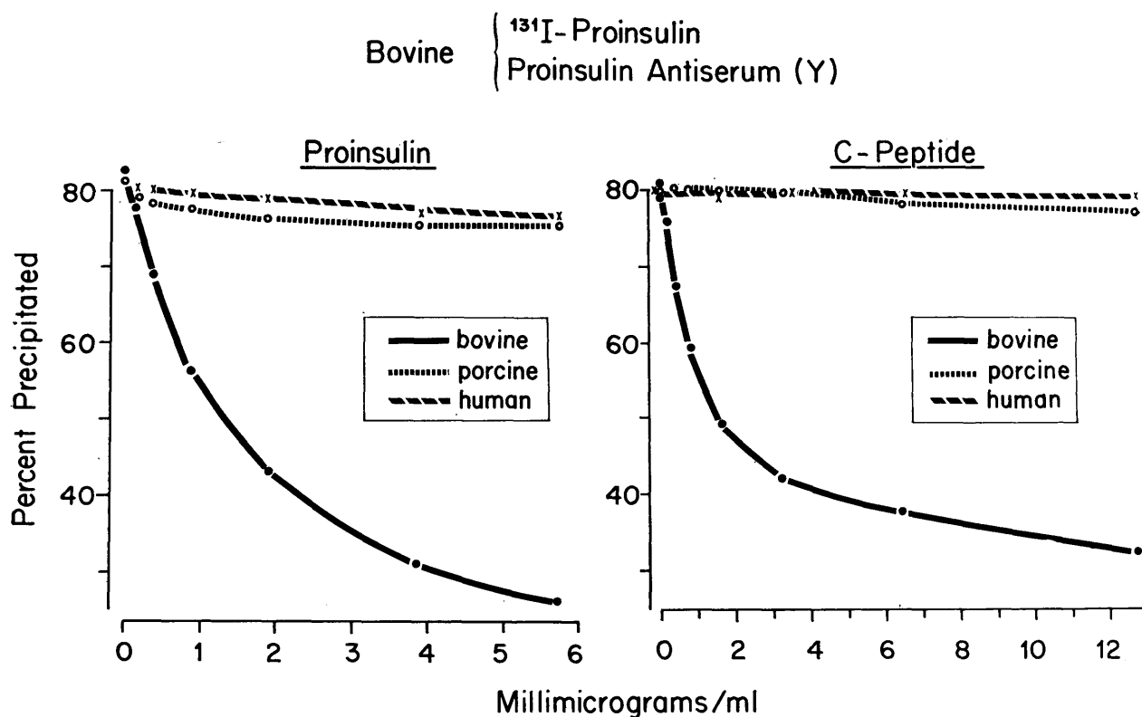
FIG. 5. Competition among bovine, porcine and human proinsulins, the respective C-peptides and bovine I-131-proinsulin for binding to antibodies in purified bovine proinsulin antiserum (Y).
