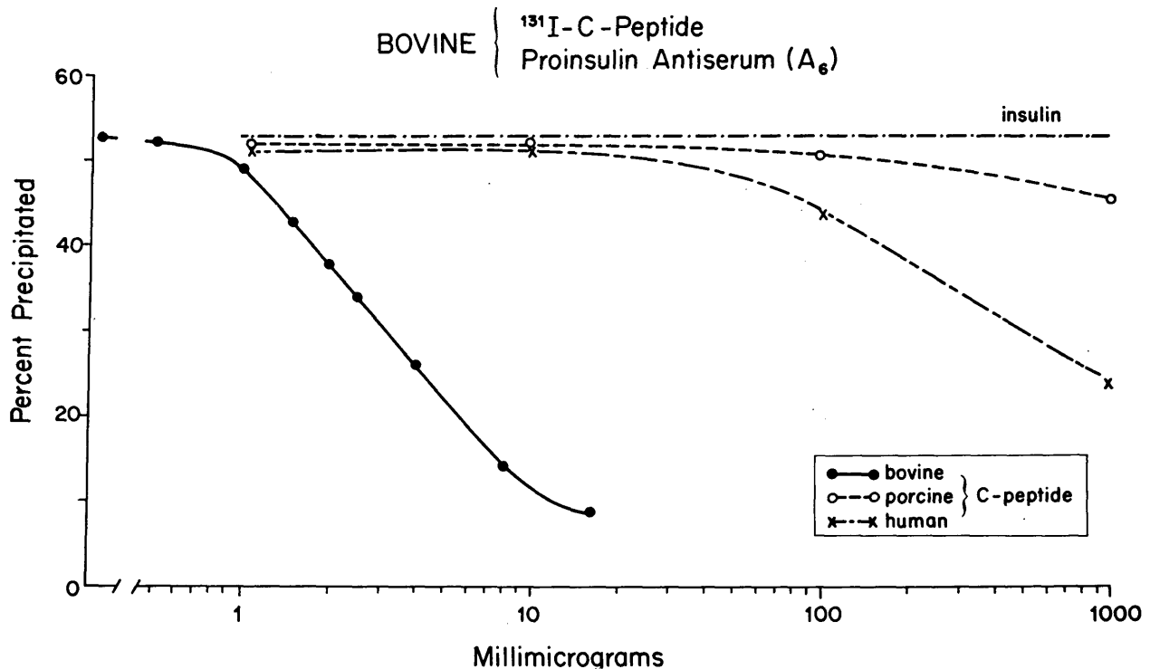
FIG. 6. Competition between increasing concentrations of C-peptides (bovine, porcine and human) and bovine I- 131 -tyrosylated C-peptide for binding sites in bovine proinsulin antiserum (A 6 ). Increasing concentrations of bovine C-peptide (1 to 10 mμg.) give a steep slope, while human and porcine C-peptides react weakly. Insulin does not react in this system.
