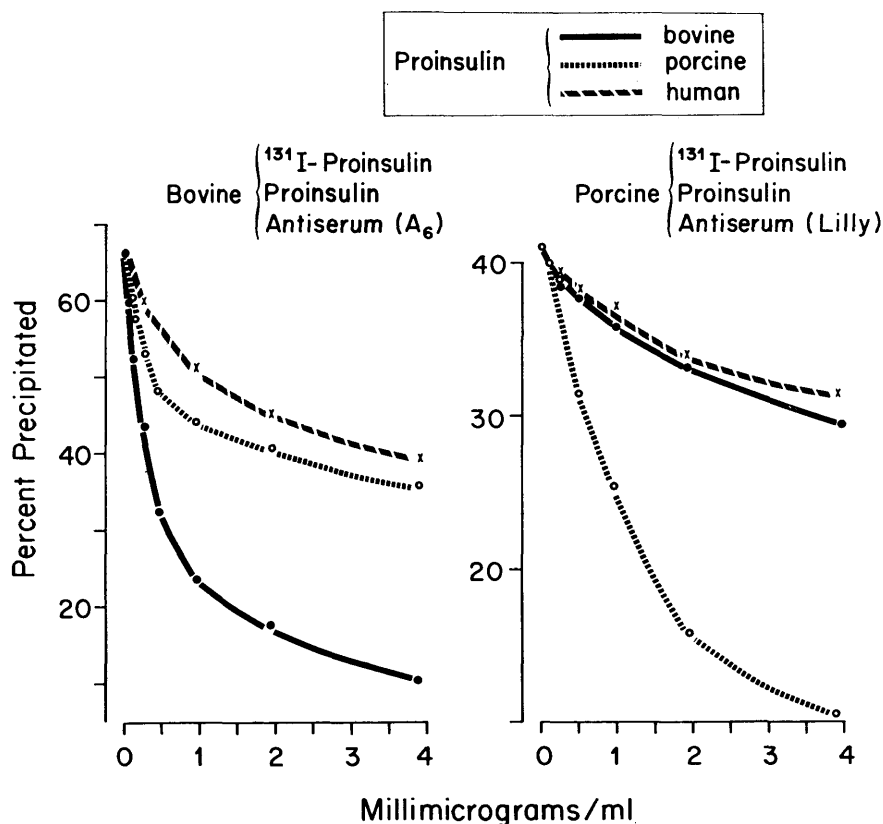
FIG. 4. Competition between increasing concentration of unlabeled proinsulin (bovine, porcine and human) and bovine I- 131 -proinsulin for binding to antibodies in bovine proinsulin antiserum (left side). The result of a similar experiment using porcine proinsulin antiserum and porcine I- 131 -proinsulin is shown on the right. In both instances, only the homologous proinsulin standard gave a steep curve.
