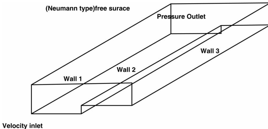
Figure 17 | Geometric alignment of flume channel along with boundary conditions.
