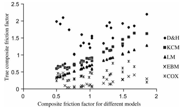
Figure 3 | True composite friction factor v/s composite friction factor predicted by five methods for Tang & Knight's (2001b) experimental conditions.
