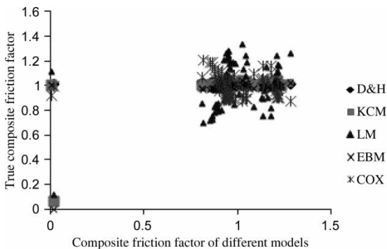
Figure 2 | True composite friction factor v/s composite friction factor predicted by five methods for Soong & Depue's (1996) experimental conditions.
