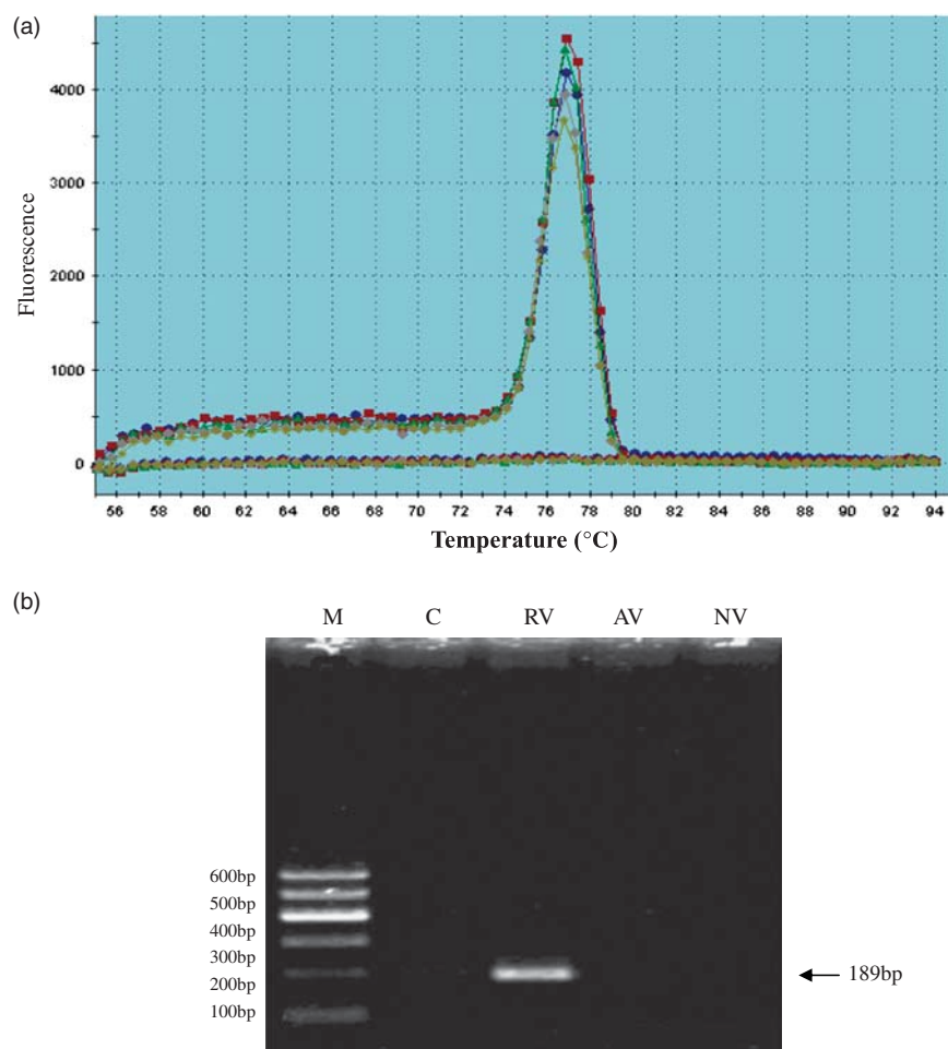
Figure 2 | Specificity of the real-time PCR: (A) melting curve analyses for RV (B) Agarose gel electrophoresis of amplified products. Lanes: M, 100 bp DNA ladder; C, negative control; RV, rotavirus; AV, Astrovirus; NV, Norovirus. The positive band denotes 189 bp products. Subscribers to the online version of Water Science and Technology can access the colour version of this figure from http://www.iwaponline.com/wst .
