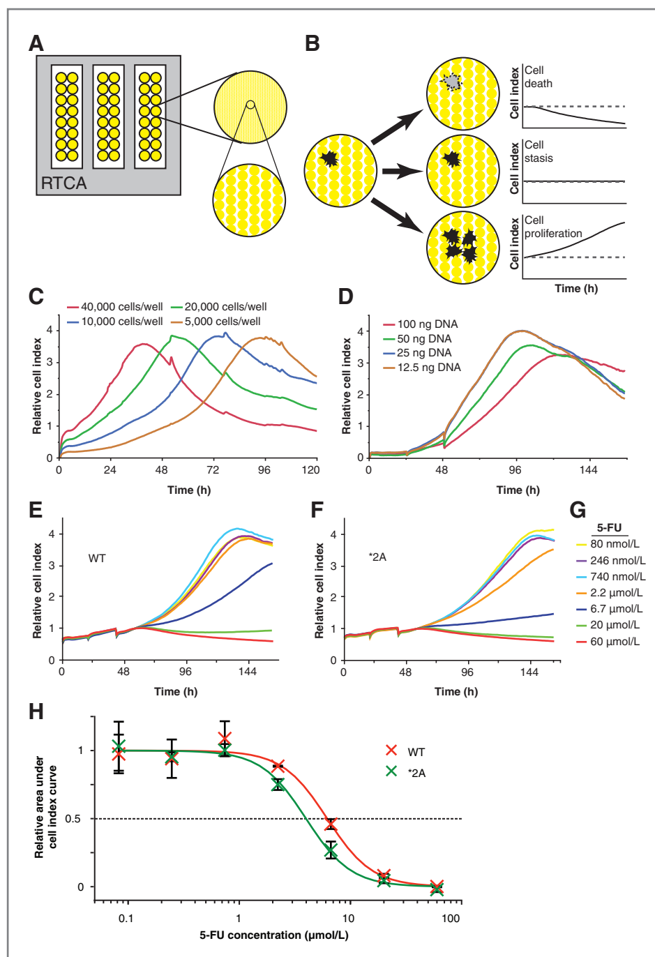
Figure 3. RTCA of variant-expressing cells treated with 5-FU. A , the surface area of RTCA plates are approximately 80% covered with gold microelectrodes used for measuring impedance. B , cells attached to the plate surface disrupt conductivity at the electrode-solution interface enabling the kinetic monitoring of changes in the cell population. C , HEK293T/c17 cells were seeded at varying densities and cell index monitored. D , cells were transfected with varying amounts of plasmid DNA (empty pIRES-neo3 vector) using a 3:1 ratio of FuGene HD to plasmid. Cells were cultured on RTCA plates for 20 hours and transfected with vectors encoding WT DPYD (WT; E ) and the catalytically inactive *2A variant ( F ). Twenty hours after transfection, cells were treated with the concentrations of 5-FU indicated ( G ). H , area under the curve was determined for each cell index profile using an analysis window defined as 8 hours to 96 hours after 5-FU treatment and IC_{50} of 5-FU was calculated. Data were rescaled relative to the maximum and minimum asymptotes for ease of visualization and are presented \pm SD of three technical replicates. Cell index profiles in C–F represent the average of three technical replicates. Data in E and F were normalized to 8 hours post-5-FU treatment using the \Delta method.
