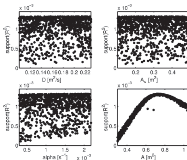
Figure 4 | Dotted plot showing the projection of the response surface, i.e. the support values (normalised and transformed coefficient of efficiency R^2 values, with higher values indicating better models), into the individual parameter dimensions: the dispersion coefficient D ; the main channel area A ; the storage zone area A_s ; and the exchange coefficient \alpha . The plot is based on a uniform random search sampling 1000 sets from the feasible parameter space.
