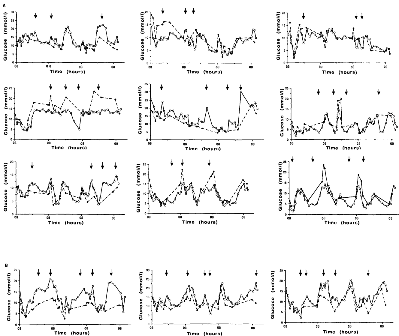
Figure A1 —Self-monitoring of blood glucose (---) and continuous microdialysis measurements of glucose in subcutaneous adipose tissue (—). Glucose profiles obtained in the remaining nine type I diabetic patients with intermediate accuracy in home glucose monitoring are shown in A, and the three remaining patients with low accuracy in self-monitoring of blood glucose are given in B. Arrows depict significant discrepancies between the two types of recordings.
