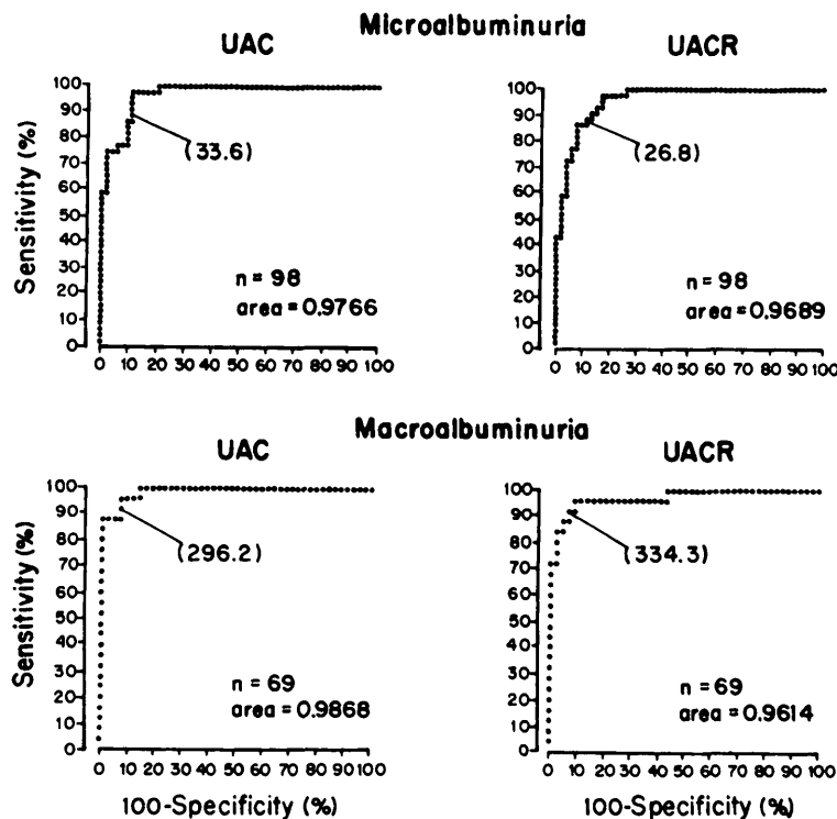
Figure 1 —ROC curves for UAC and UACR as a screening test for microalbuminuria and macroalbuminuria. Values in parentheses (UAC = mg/l; UACR = mg/g) correspond to the intersection of the curve with the 100%-to-100% diagonal.
