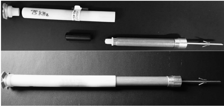
FIGURE 1. (top) Disassembled dart showing individual pieces and transmitter. The magnet placed on the outer housing is effective at shutting off the transmitter when not in use. (bottom) Fully assembled dart with the magnet removed is ready to fire.
