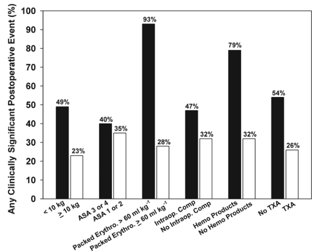
Fig. 3. Percentage of any clinically significant postoperative event requiring intensive care unit admission for the multivariate risk factors identified. Clinically significant postoperative event = cardiorespiratory and/or hematological event. The multivariate risk factors include body weight <10 kg, ASA class 3 or 4, packed erythrocyte transfusion >60 ml/kg, intraoperative complication, hemostatic blood product transfusion (platelets, fresh-frozen plasma, and/or cryoprecipitate), and tranexamic acid (TXA) not given. ASA 3 or 4 = American Society of Anesthesiologists physical status 3 (a patient with severe systemic disease) or 4 (a patient with severe systemic disease that is a constant threat to life); Hemo. Products = platelets, fresh-frozen plasma, and/or cryoprecipitate; Intraop. = intraoperative; Intraop. Comp. = intraoperative complication (refer to the appendix for detailed definition); Packed Erythro = intraoperative packed erythrocyte transfusion.
