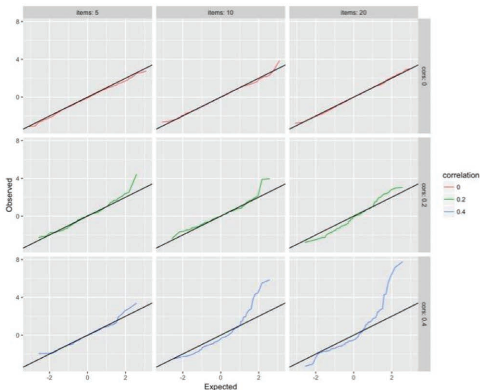
Fig. 2. Selected results from the simulations used to evaluate the Carlisle Method. If the expected distribution from the sum of P values from a trials report's "table 1" ( x -axis) is the same as the observed distribution of P values ( y -axis), the test values (colored lines) will fall directly on the diagonal black line. Departures from the black line indicate false-positives as the observed distributions exceed what is expected by chance. When the correlation between items is 0 (top row), the Carlisle Method performs well. However, as the degree of correlation (rows) increases, many false positives are observed. This effect is amplified with increasing number of items (columns) in the table.
