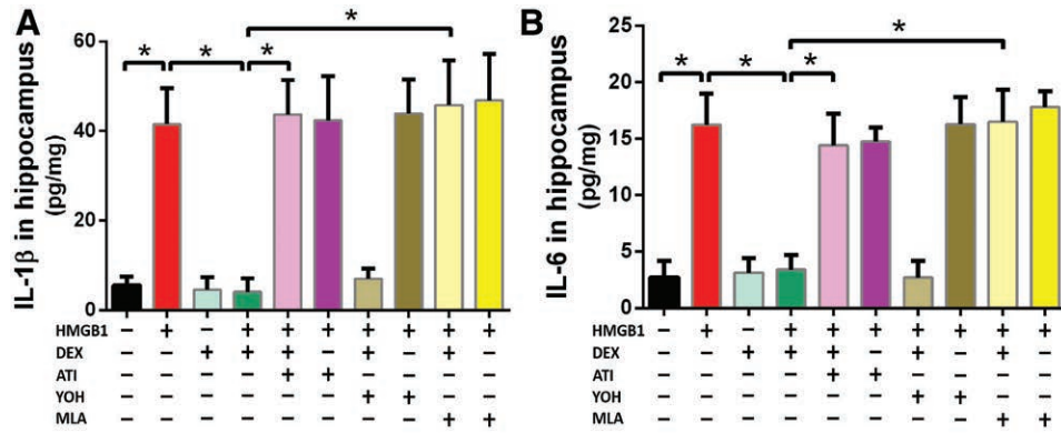
Fig. 4. Dexmedetomidine prevents high mobility group box 1 protein (HMGB1)–induced hippocampal inflammation in an atipamezole- and methyllycaconitine-sensitive manner. Ten groups of randomly assigned mice (n = 8/group) were administered antagonists (methyllycaconitine, atipamezole, yohimbine) before HMGB1 in the presence or absence of dexmedetomidine. Twenty-four hours after HMGB1, mice were euthanized, and the hippocampus was harvested and assayed by ELISA for interleukin (IL)-1β (A) and IL-6 (B). Data are expressed as means ± SD and were analyzed by one-way ANOVA and Tukey post hoc test. *P < 0.0001 for comparisons shown.
