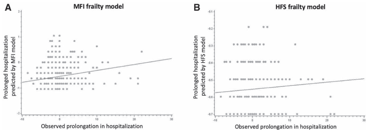
Fig. 4. Calibration plots of Modified Frailty Index (MFI, A) and Hopkins Frailty Score (HFS, B) models (N = 1,042).
