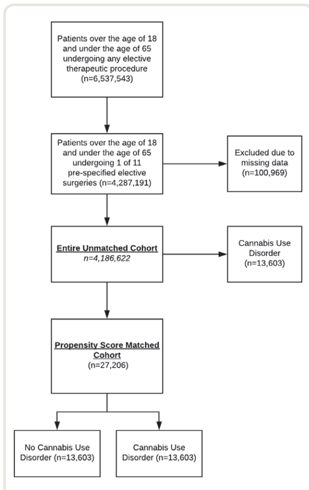
Fig. 1. Flowchart demonstrating cohort formation.
