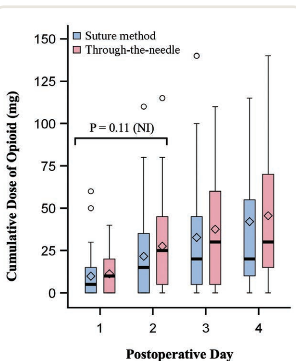
Fig. 6. Effects of the suture versus through-the-needle catheter on postoperative opioid consumption over time. Data are expressed as mean (diamond) and median (horizontal bar) with 25th through 75th (box); whiskers extend to the most extreme observations within 1.5 times the interquartile range of the first and third quartiles, respectively; circles represent outliers.
