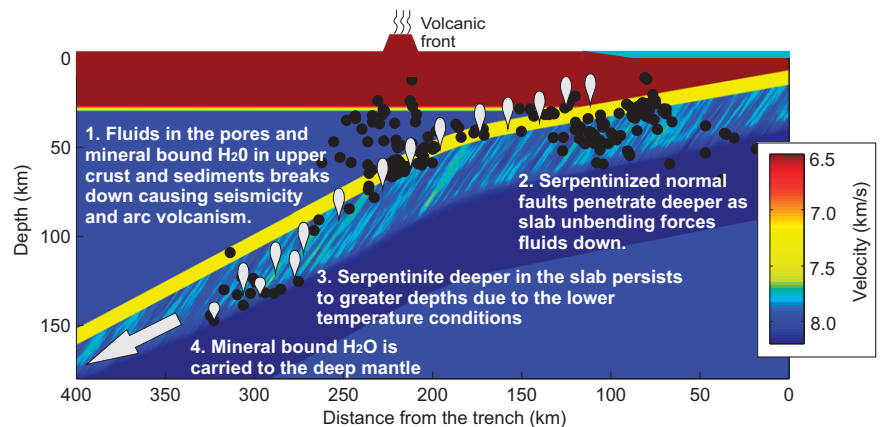
Figure 4. Summary of subduction zone structure inferred for waveform modeling of dispersed P-wave arrivals. Hydration of slab mantle is described by von Kármán function, which provides large-scale elongate structures representing normal fault structures inferred. Smaller scale structures are required to provide observed P-wave coda. Fault depth increase with distance from outer rise is due to downward forcing of fluids (Faccenda et al., 2009, 2012). Black dots show Wadati-Benioff zone (northern Japan) seismicity. Approximate depth at which mineral-bound water is released is shown by white balloon shapes. Some mineral-bound water is delivered to mantle transition zone (e.g., Rüpke et al., 2004; Savage, 2012), indicated by white arrow. Depth of penetration of these hydrated fault zone structures is controlled by temperature at which serpentine is stable. As slab is heated at depth, stability field of serpentine becomes restricted to cool core of slab.
