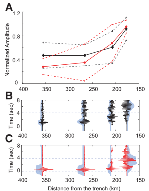
Figure 3. A: Scattering analysis for all events with observed coda decay (black) compared to modeled coda decay (red). Plot shows average coda ratio normalized to maximum coda ratio for given event. B: Observed high-frequency (>3.0 Hz) P-wave arrivals with extended coda (black); coda envelope is plotted in blue. C: Synthetic P-wave arrivals (high pass filtered at 3.0 Hz) from numerical model incorporating elongated random scatterers in Wadati-Benioff zone (northern Japan). (Example of von Kármán scattering medium is shown in Fig. 4; actual model is shown in Fig. DR4b [see footnote 1].)
