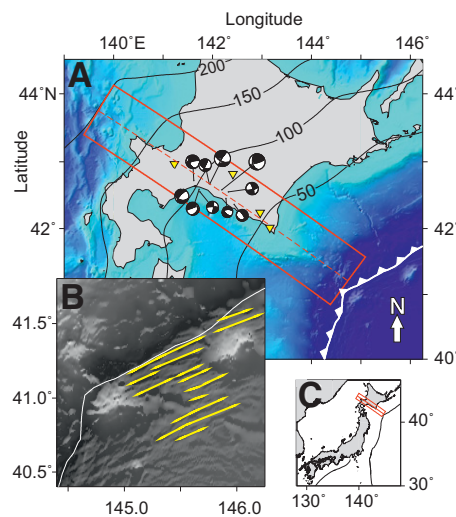
Figure 1. Summary map of Wadati-Benioff zone of northern Japan. A: Focal mechanisms (in black and white) of earthquakes used in full waveform analysis; stations are shown by yellow triangles. Black contours show depth to slab (Hayes et al., 2012). B: Outer rise fault scarps, highlighted in yellow, in Japan subduction zone trench. Bathymetry is from Gebco08 model (General Bathymetric Chart of the Oceans; www.gebco.net ). C: Location map of study area. Red box shows profile area described in this study.
