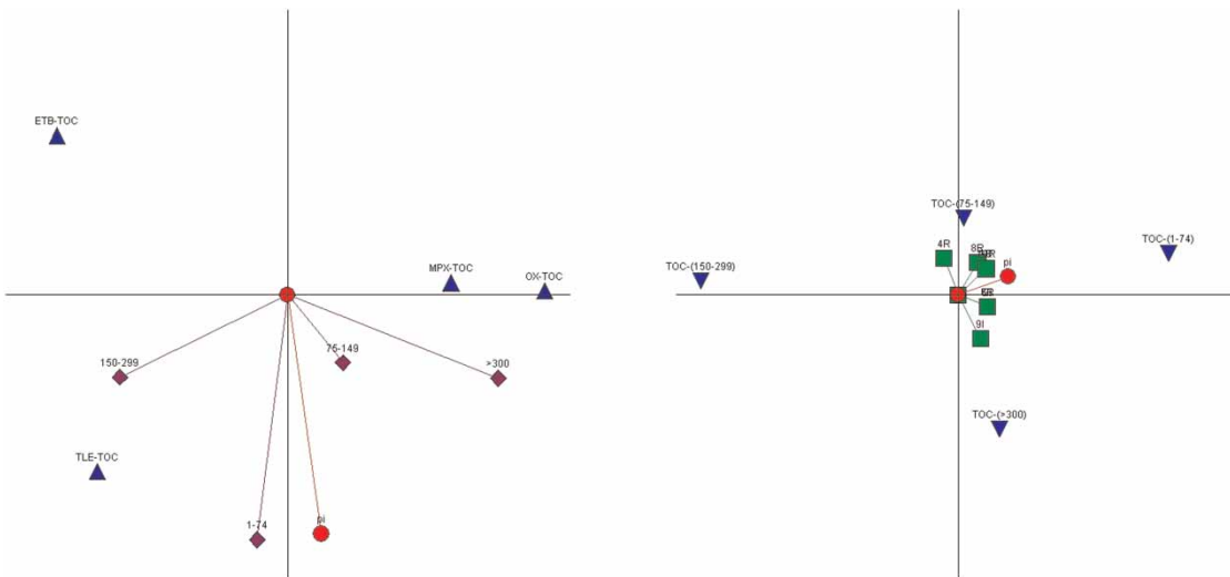
Figure 11 | GAIA biplot for predominant volatile organics particulate fraction (◆); (●) pi-decision axes; (▲) organics' affinity towards predominant chemical parameter; (■) study sites; (▼) TOC's presence in particulate fractions.
