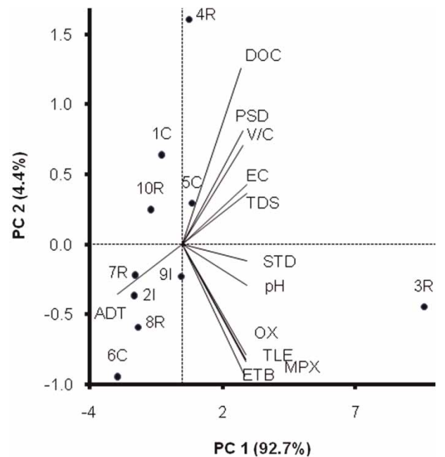
Figure 7 | PCA biplot for volatile organics build-up on urban roads at <1\mu\text{m} fractions (objects are represented with numbered labels with suffix C = commercial, I = Industrial or R = residential).
