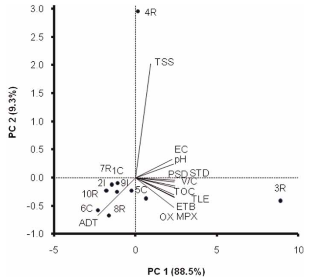
Figure 6 | PCA biplot for volatile organics build-up on urban roads at 75–149 \mu\text{m} fractions (objects are represented with numbered labels with suffix C = commercial, I = Industrial or R = residential).
