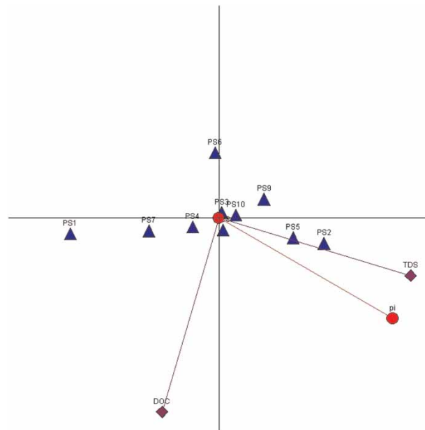
Figure 9 | GAIA biplot for predominant chemical parameter scenario (◆) for the dissolved heavy metals; (●) pi-decision axis; (▲) <1 µm fraction.
