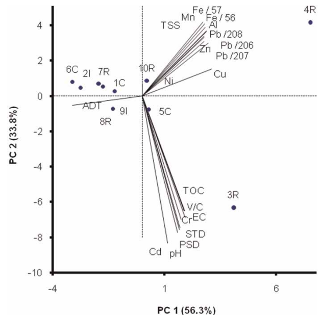
Figure 3 | PCA biplot for heavy metals build-up on urban roads at 1–74 μm fractions (objects are represented with numbered labels with suffix C = commercial, I = industrial or R = residential).
