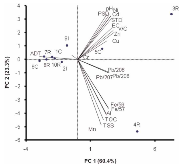
Figure 2 | PCA biplot for heavy metals build-up on urban roads at 150–299 μm fractions (objects are represented with numbered labels with suffix C = commercial, I = industrial or R = residential).
