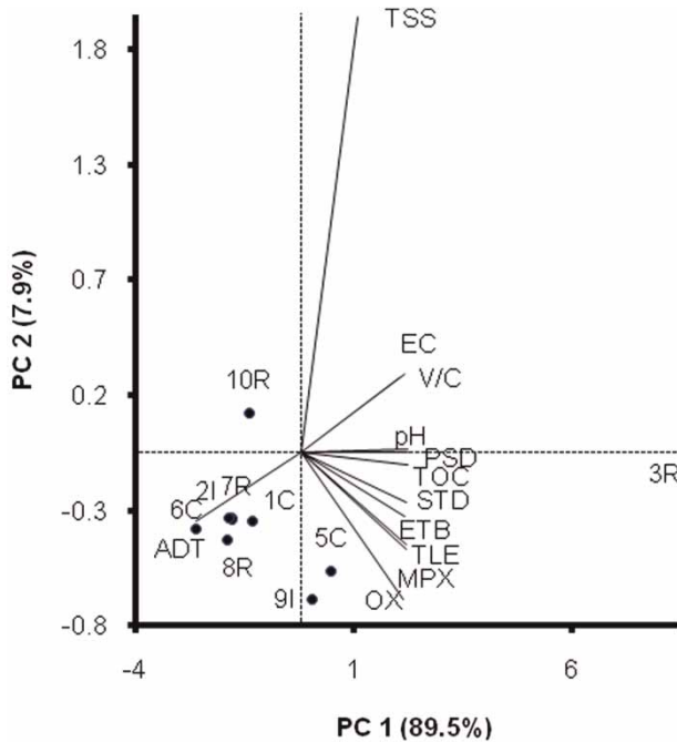
Figure 5 | PCA biplot for volatile organics build-up on urban roads at >300\mu\text{m} fractions (objects are represented with numbered labels with suffix C = commercial, I = Industrial or R = residential).
