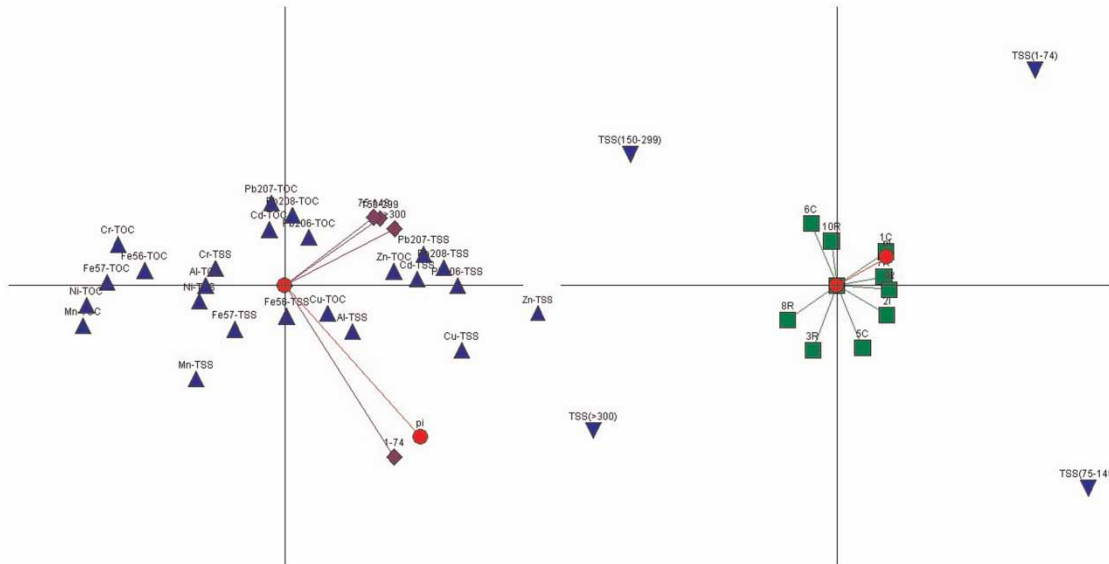
Figure 10 | GAIA biplot for predominant heavy metals particulate fraction (◆); (●) pi-decision axes; (▲) metals' affinity towards predominant chemical parameters; (■) study sites; (▼) TSS' presence in particulate fractions.
