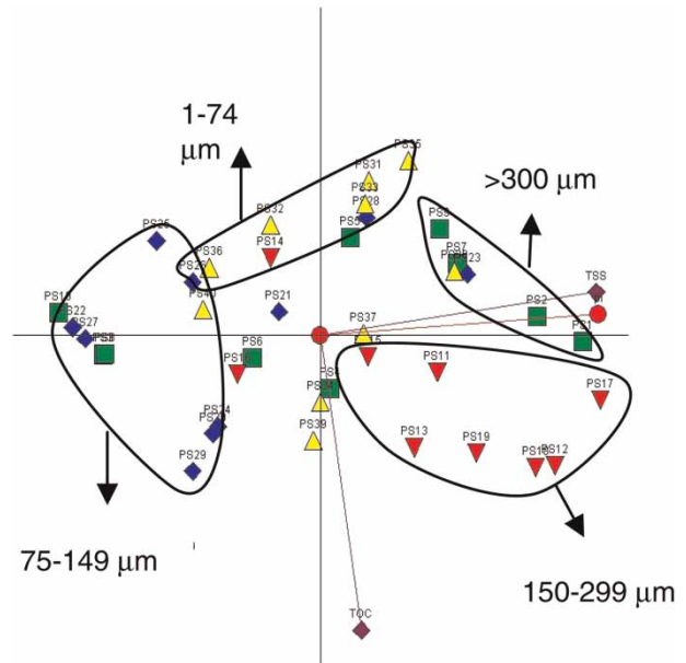
Figure 8 | GAIA biplot for predominant chemical parameter scenario (◆) for particulate heavy metals; (▼) pi-decision axis; (▲) >300 µm fractions; (▼) 150-299 µm fractions; (◆) 75-149 µm fractions; (▲) 1-74 µm fractions.
