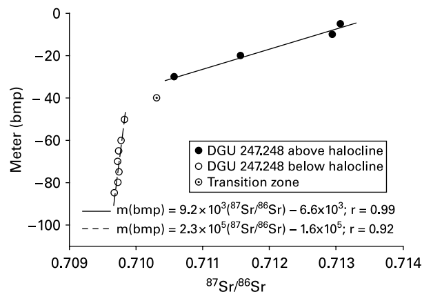
Figure 11 | The ^{87}\text{Sr}/^{86}\text{Sr} ratio distributions with depth in groundwater samples collected from well DGU 247.248, Neksø Municipal Waterworks.
