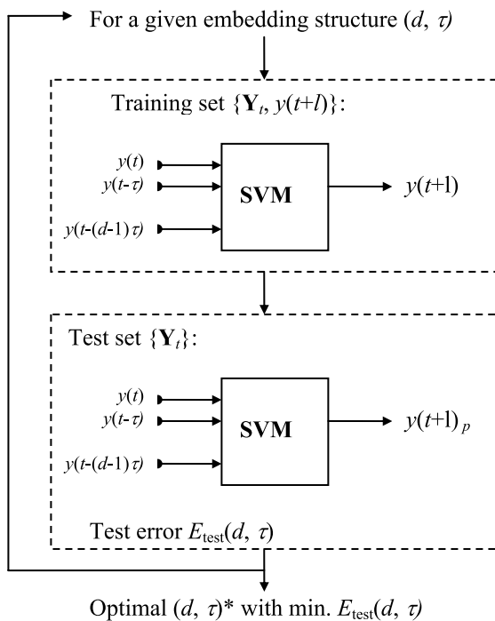
Figure 3 | Algorithm for the optimal algorithm used in optimal embedding structure search.
