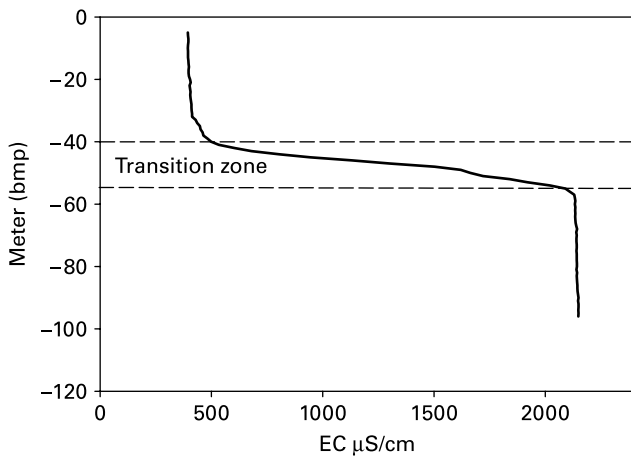
Figure 3 | Electrical conductivity log of well DGU 247.248, Neksø Municipal Waterworks. Note the significant halocline at 40–55 m bmp.
