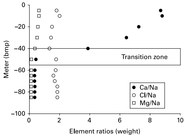
Figure 6 | Variations with depth of selected element/Na ratios in well DGU 247.248.
