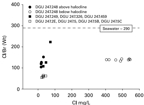
Figure 7 | Cl/Br (weight) ratios vs. Cl contents of water samples from well DGU 247.248 and other production boreholes in the well field of Neksø Municipal Waterworks. The Cl/Br (weight) ratio of normal oceanic seawater is shown for comparison.
