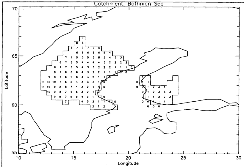
Fig. 4. Bothnian Sea. The numbers correspond to the gridboxes of the model catchment and express the flow distance in gridboxes from the inflow box (= 0) into the Baltic Sea. The thick line represents the border of the real catchment derived from a dataset (Hagemann and Dümenil 1998).
