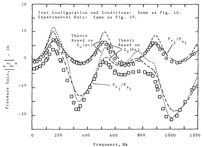
Fig. 11 Effect of orifice resistance on theoretical pressure gain
