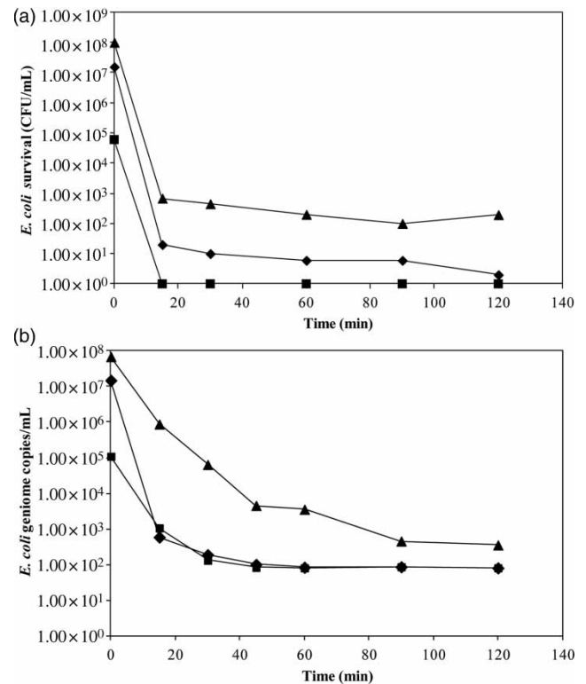
Figure 2 | E. coli inactivation in water samples containing various initial bacterial concentrations during PEC (2V potential), assessed by (a) the culture technique and (b) qPCR.
