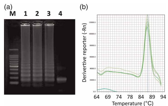
Figure 2 | The specificity of LAMP products. (a) LAMP products obtained from 10 \text{ pg} of M. avium 104 DNA (Lane 1) and from nucleic acid extracts of pure cultures of M. avium 104 on the FTA elute cards (approximately 10^8 and 10^7 cells, Lanes 2 and 3, respectively), and restriction digestion of the products obtained from 10 \text{ pg} of M. avium 104 DNA with TaqI (bands corresponding to 171 and 163 bp are expected, Lane 4). (b) The peaks of melting temperature curves of LAMP products amplified from control M. avium 104 DNA coincided with those from five isolates of environmental M. avium . Products from all isolates had a melting temperature of 87.3^\circ\text{C} .
