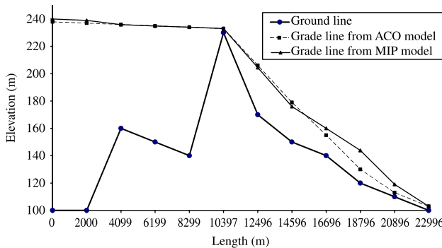
Figure 6 | Longitudinal profile of the path and the steady state grade lines resulted from ACO and MIP models (second example).
