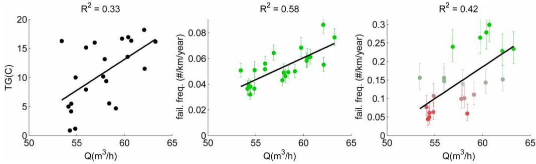
Figure 6 | Correlation between water consumption and mean temperature (left panel), water consumption and pipe failure for AC pipes (middle panel), and for steel pipes (right panel). Water consumption is represented by the flow rate Q .
