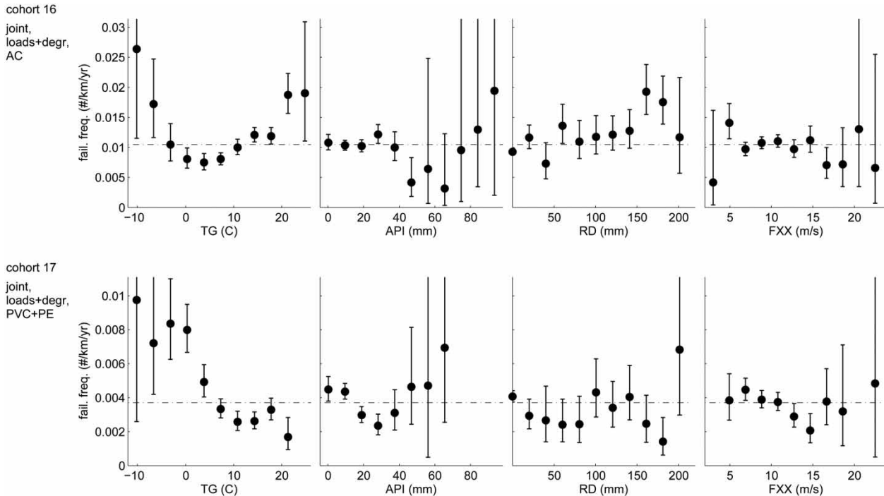
Figure 5 | Failure frequency as a function of weather variables (temperature, drought, wind) for different joint cohorts using the frequency analysis. Each point represents a number of failures over a fixed interval of the weather variable. Error bars indicate the 80% confidence intervals.
