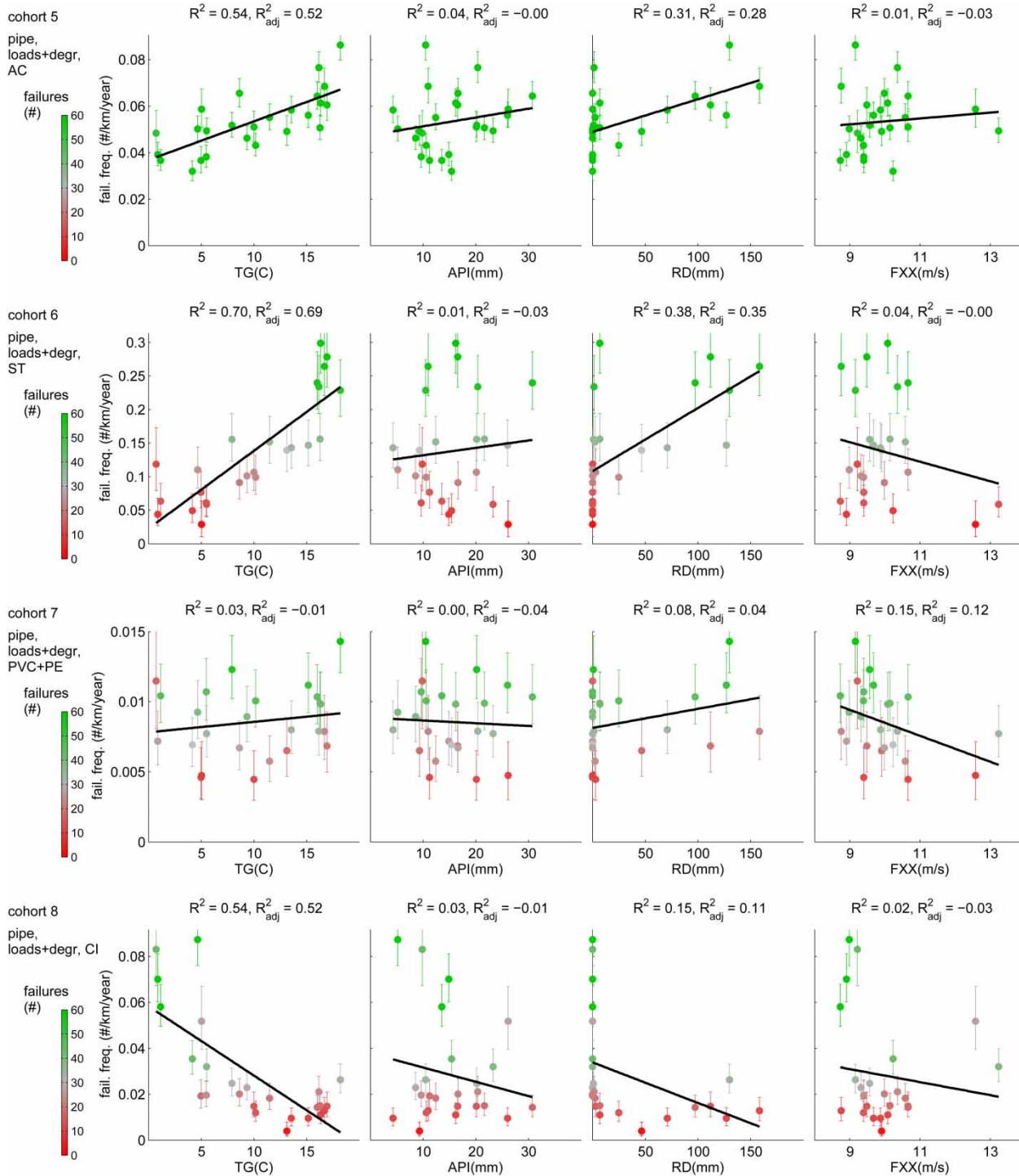
Figure 3 | Failure frequencies as a function of weather variables (temperature, drought, wind) for different pipe material cohorts. Each point represents a 2-month period. Error bars indicate the 80% confidence intervals. The number of failures is indicated using a scale.
