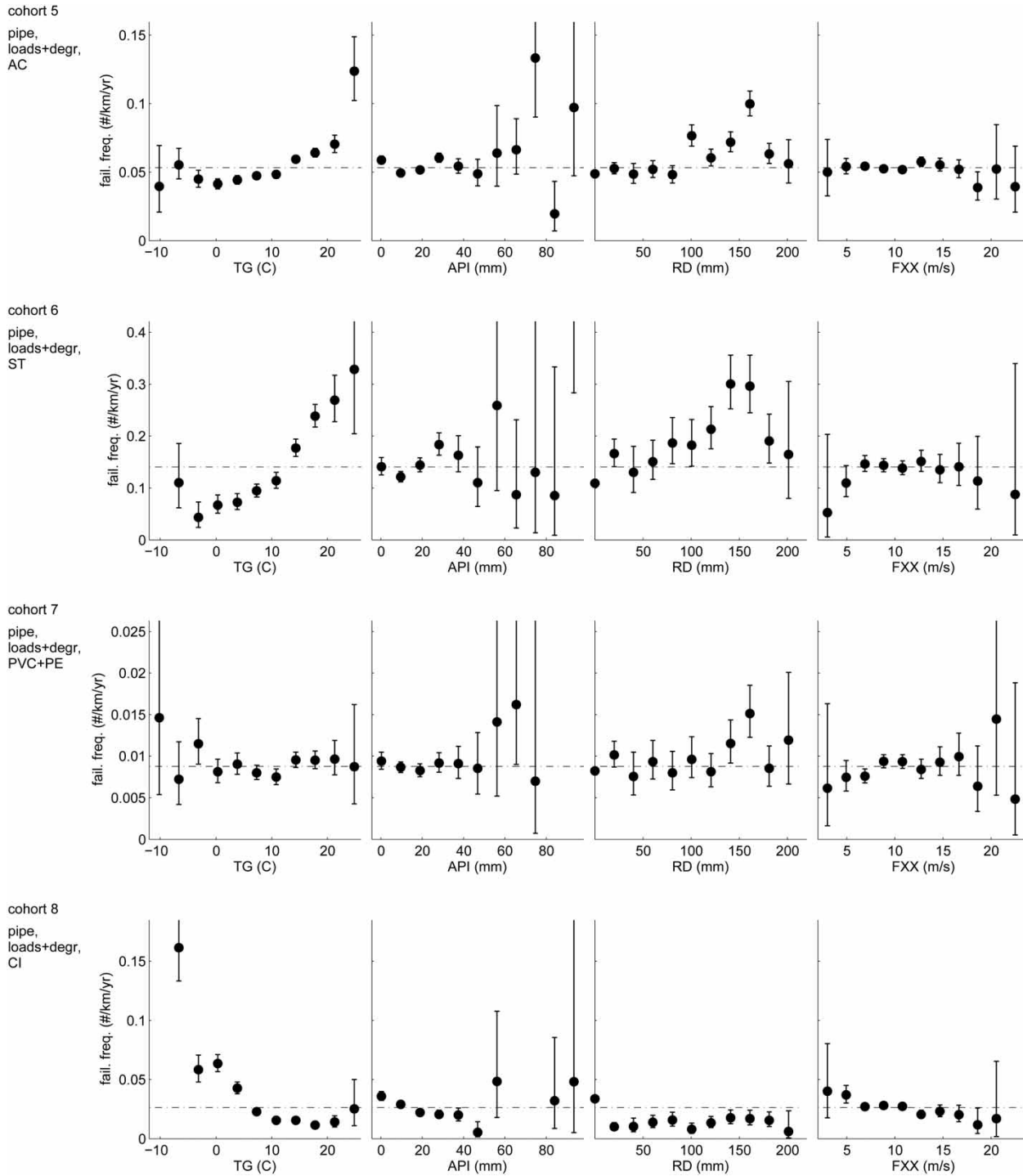
Figure 4 | Failure frequency as a function of weather variables (temperature, drought, wind) for different pipe material cohorts using the frequency analysis. Each point represents a number of failures over a fixed interval of the weather variable. Error bars indicate the 80% confidence intervals.
