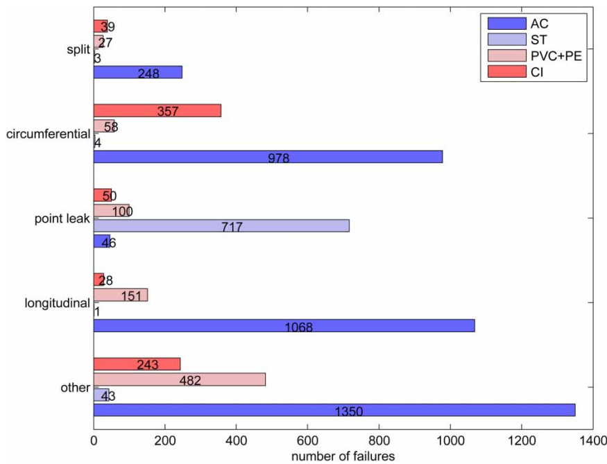
Figure 7 | Type of failures for the different pipe materials registered by USTORE.
