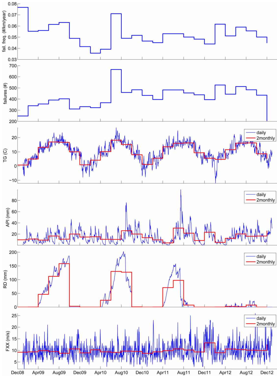
Figure 2 | Time series of failure data and weather data on daily and monthly basis. During the year 2009 the number of failures increased (whereas the failure frequency decreased), because more water companies registered their failure data.
