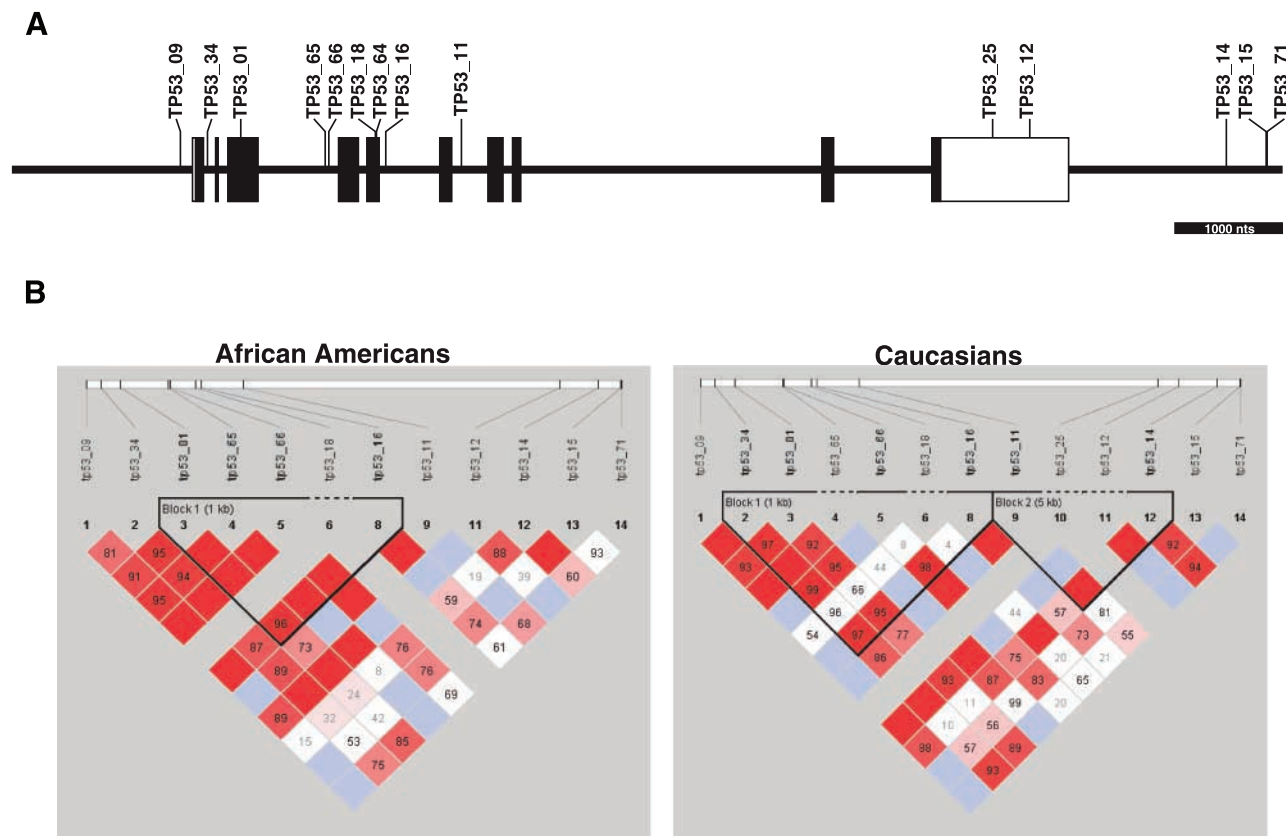
Figure 1. Position and linkage of haplotype tagging polymorphisms in TP53 . A , diagram of the TP53 gene and the position of polymorphisms genotyped. Figure was generated using SNP map ( http://www.drgang.net/svg_map.html ). Polymorphisms are labeled according to National Cancer Institute Core Genotyping Facility nomenclature ( http://snp500cancer.nci.nih.gov ). Corresponding rs numbers are listed in Supplementary Table S1. Filled boxes , coding exonic regions; empty box , noncoding region of the exon. Line , intronic regions. B , graphical representation of D' values for TP53 polymorphisms was generated for case-control participants using Haploview (30) and the block definitions from Gabriel et al. (31).
