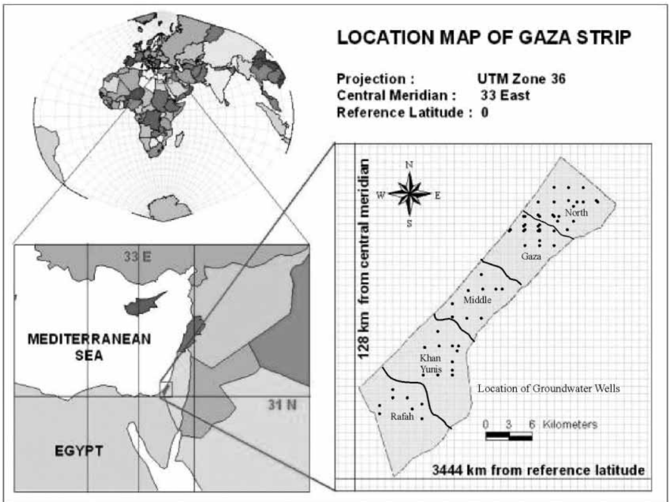
Figure 1 | Five regions of the Gaza Strip and location of groundwater wells.
