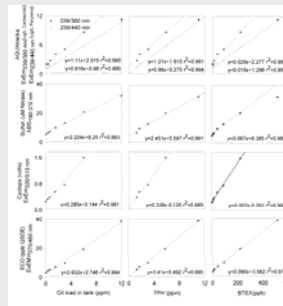
Figure 4. Regression equations for estimating [oil] (TPH and BTEX) from in situ sensors.
