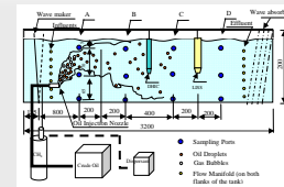
Figure 9. Schematic representation (in cm, not to scale) of flow-through wave tank with subsea injection system.
