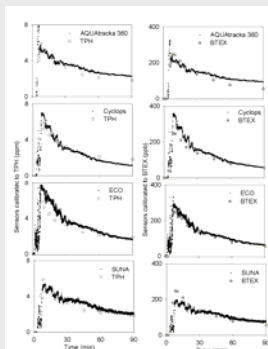
Figure 8. Estimated (sensors) and measured oil (TPH & BTEX) concentrations during simulated oil plume dilution with RAPID decay.
