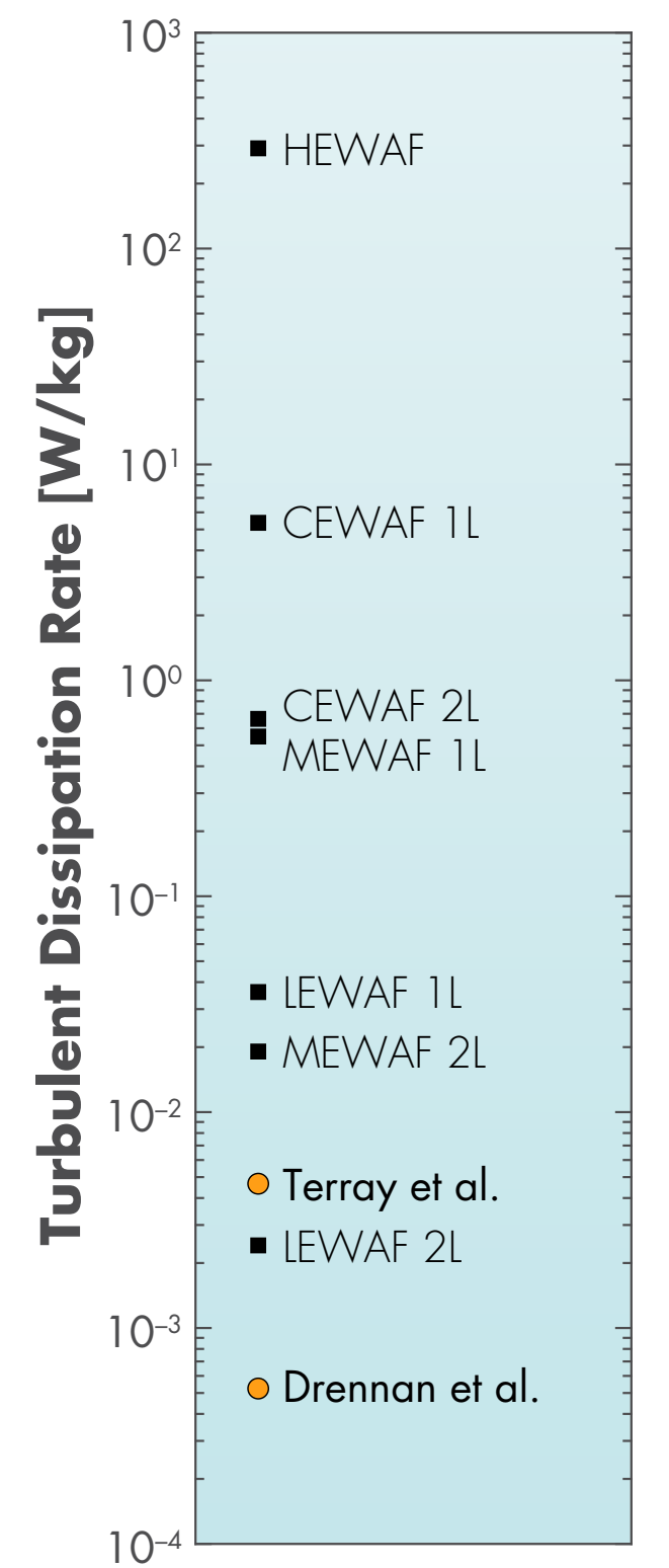
Figure 4. Plot of the measured turbulent dissipation rate from this study alongside measurements from prior work.
