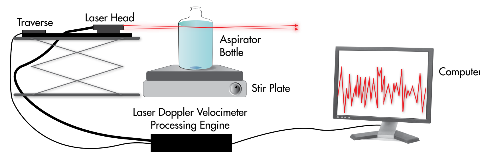
Figure 2. Schematic representation of the experimental setup. The aspirator bottle or blender jar is measured by the Laser Doppler Velocimeter (LDV). The computer records this data for further processing.
