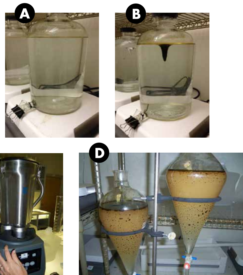
Figure 1. Examples of LEWAF (A), MEWAF (B), and HEWAF (C,D) preparations in the laboratory
