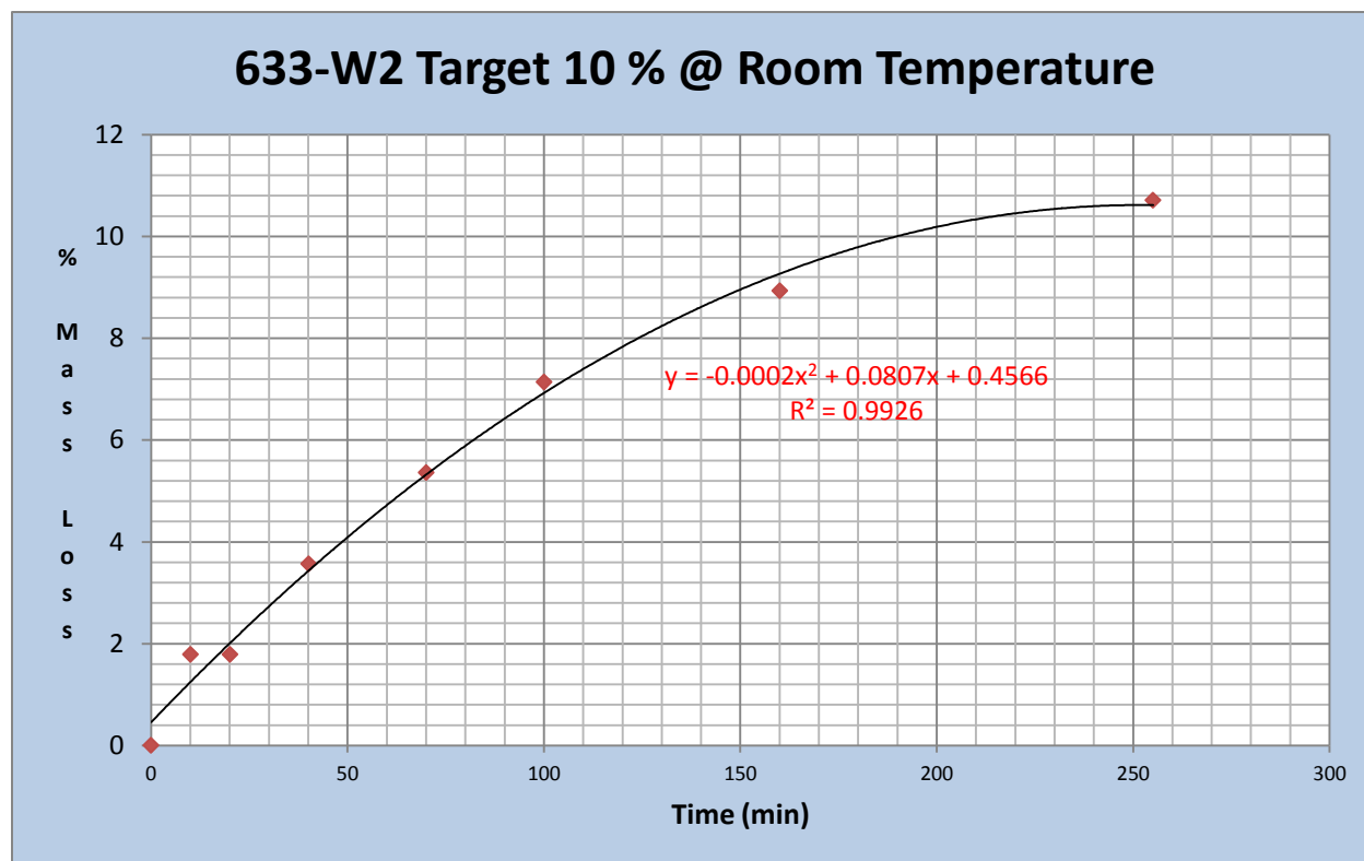
Figure 1. Mass loss to approximately 10% over time of HOOPS crude oil exposed to air sparging at 1 L/min in the lab at approximately 20 °C.
