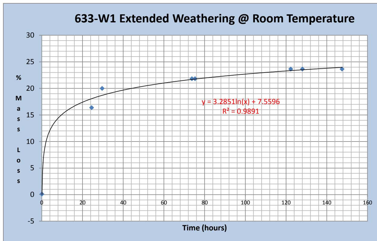
Figure 2. Mass loss of HOOPS crude oil over extended time (148 hours) with air sparging at 1 L/min in the lab at 20 °C (room temperature).
