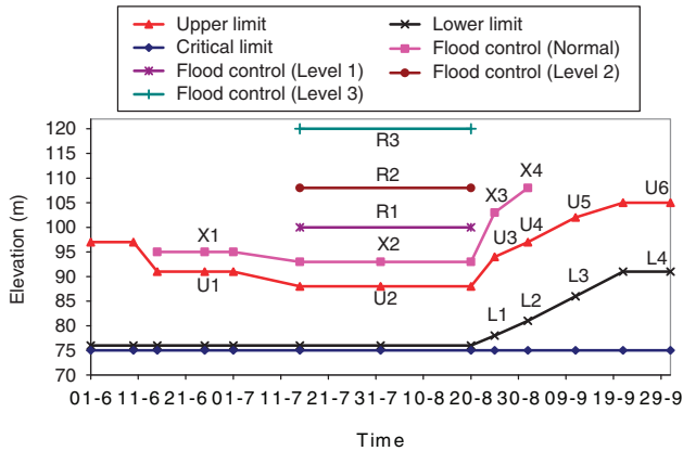
Figure 2 | Present reservoir rule curves representing reservoir water levels for flood control and hydropower generation (Ngo et al. 2007).
