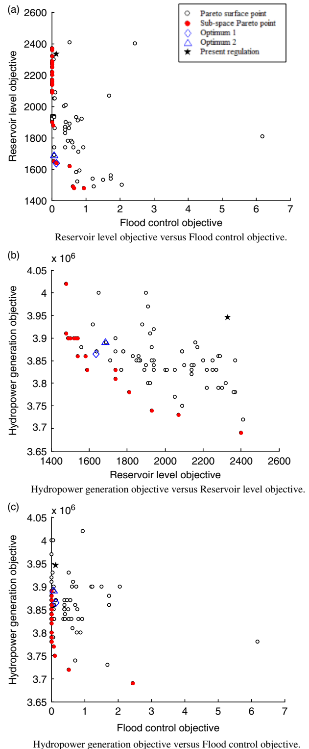
Figure 7 | Representation in 2D the sub-spaces of the 3D Pareto surface. The 78 Pareto points from the rule curve optimisation are shown in these plots. In each sub-space the Pareto front is enlightened as well as Optimum 1, Optimum 2 and the evaluation of the present regulation.
