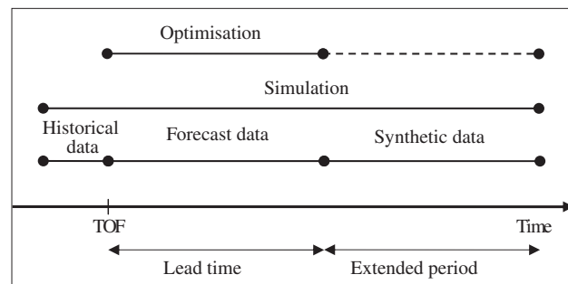
Figure 5 | Simulation-optimisation approach for real-time optimisation.
