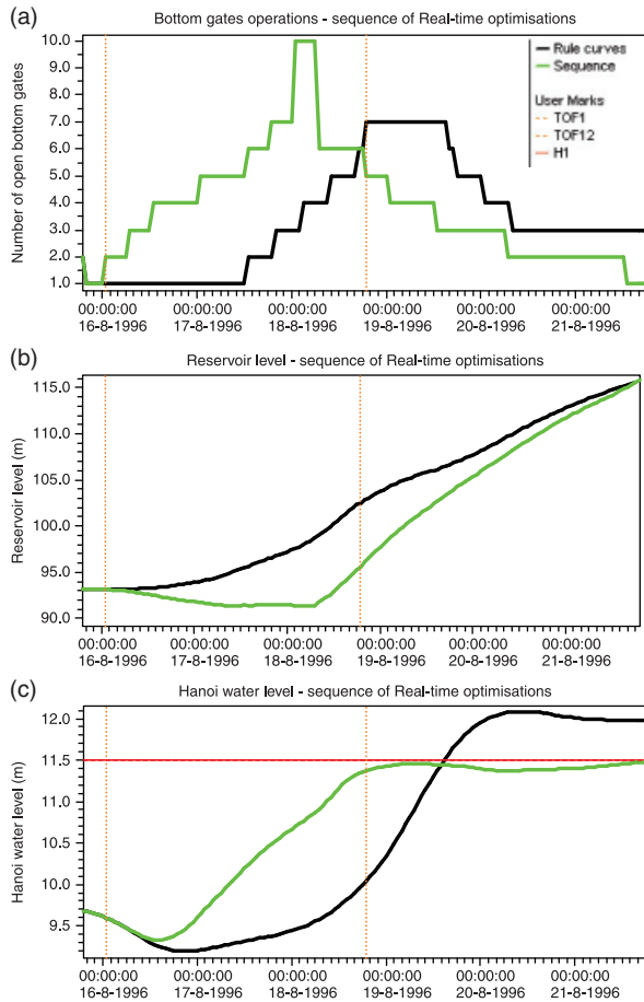
Figure 9 | Reservoir operation during the sequence of real-time optimisations under flood control operation: (a) operations of the bottom sluice gates, (b) reservoir level, and (c) water level at Hanoi. TOF1 and TOF12 are respectively the time of forecast used for the first and the twelfth run. H1 is the target water at Hanoi.
