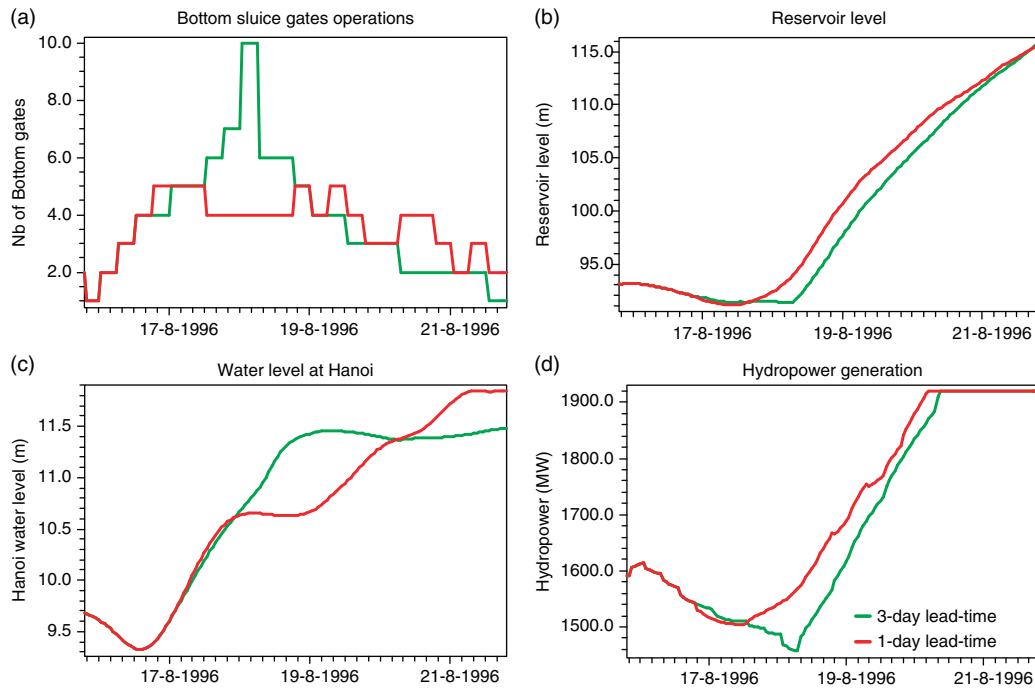
Figure 10 | Comparison of real-time operations with 3-day and 1-day flow forecasting: (a) Bottom sluice gates operation, (b) Reservoir level, (c) Water level at Hanoi and (d) Hydropower generation.
