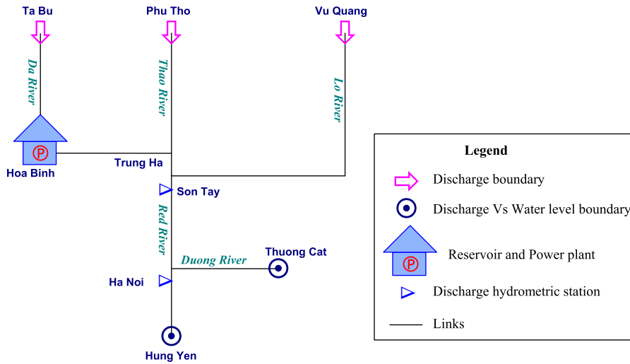
Figure 4 | MIKE 11 model setup of the lower Red River basin, including the Hoa Binh reservoir (Ngo et al. 2008).
