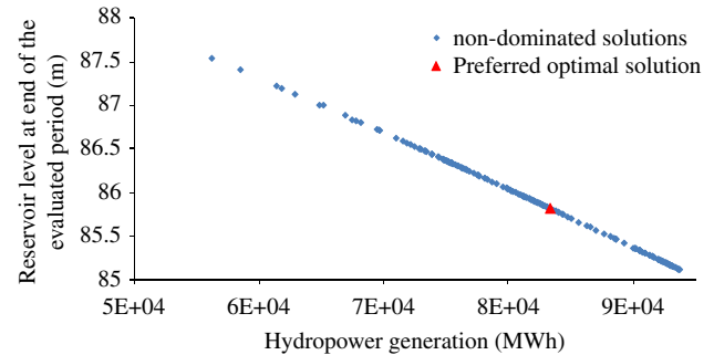
Figure 8 | Hydropower generation versus reservoir level at the end of the forecast period for the Pareto optimal solutions of the real-time optimisation under normal operation.
