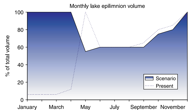
Figure 2 | Calibrated (dotted line) and estimated (filled area) future monthly lake epilimnion volume. Future estimates were based on simulation with the CE-Qual-W2 model run with the HCA2 scenarios for temperature, wind, radiation and relative humidity for Lake Kolbotnvatn (Tjomsland & Rohrlack 2008). 100% epilimnion volume denotes complete mixing of the lake.
