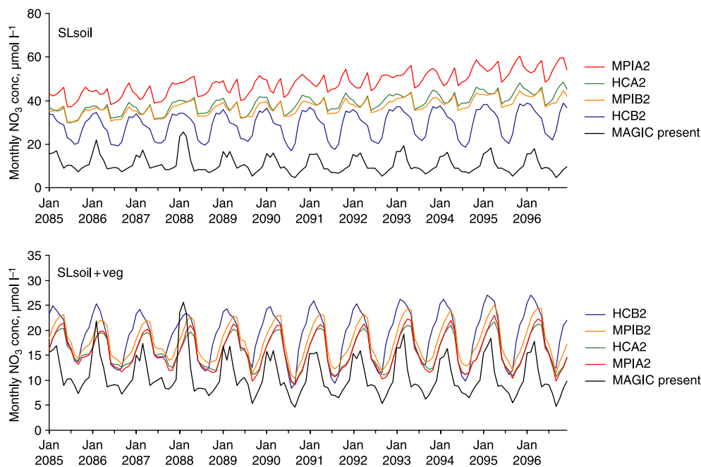
Figure 6 | Simulated monthly seasonal NO 3 surface water pattern for SLsoil (upper panel) and SLsoil + veg (lower panel) during the scenario period 2085–2096 for the different scenarios (coloured lines) compared to present-day simulations during 1993–2004 (black line). Green, blue, red and orange lines represent HCA2, HCB2, MPIA2 and MPIB2 scenarios, respectively. Units are in \mu\text{mol l}^{-1}\text{year}^{-1} . Note different scaling on the y axis. See text for details.
