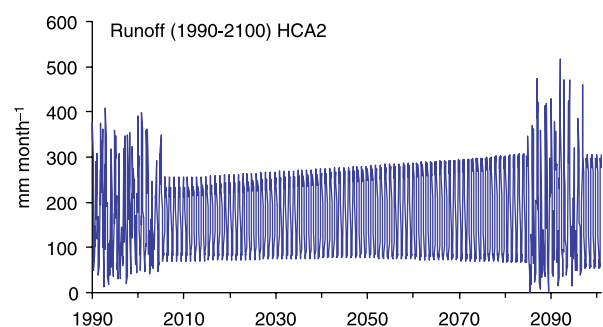
Figure 1 | Estimated runoff (mm month -1 ) during 1990–2100, exemplified for the HCA2 scenario. Measured short-term variations in runoff (1990–2004) were superimposed on a long-term linear trend, according to scenario estimates for precipitation less evaporation. See text for details.
