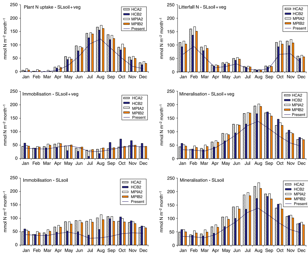
Figure 4 | Twelve-year mean monthly plant N uptake, litter fall N, immobilization and mineralization for the present-day (solid line) and the four scenario estimates of storylines SLsoil and SLsoil + veg, respectively. For SLsoil there was assumed no change in plant N uptake and litter N; thus all scenarios were assumed equal to present day. Mineralization and immobilization are results of the MAGIC simulations. Striped, black, white and grey bars represent HCA2, HCB2, MPIA2 and MPIB2 scenarios, respectively. Units are in \text{mmol N m}^{-2} \text{ month}^{-1} .
