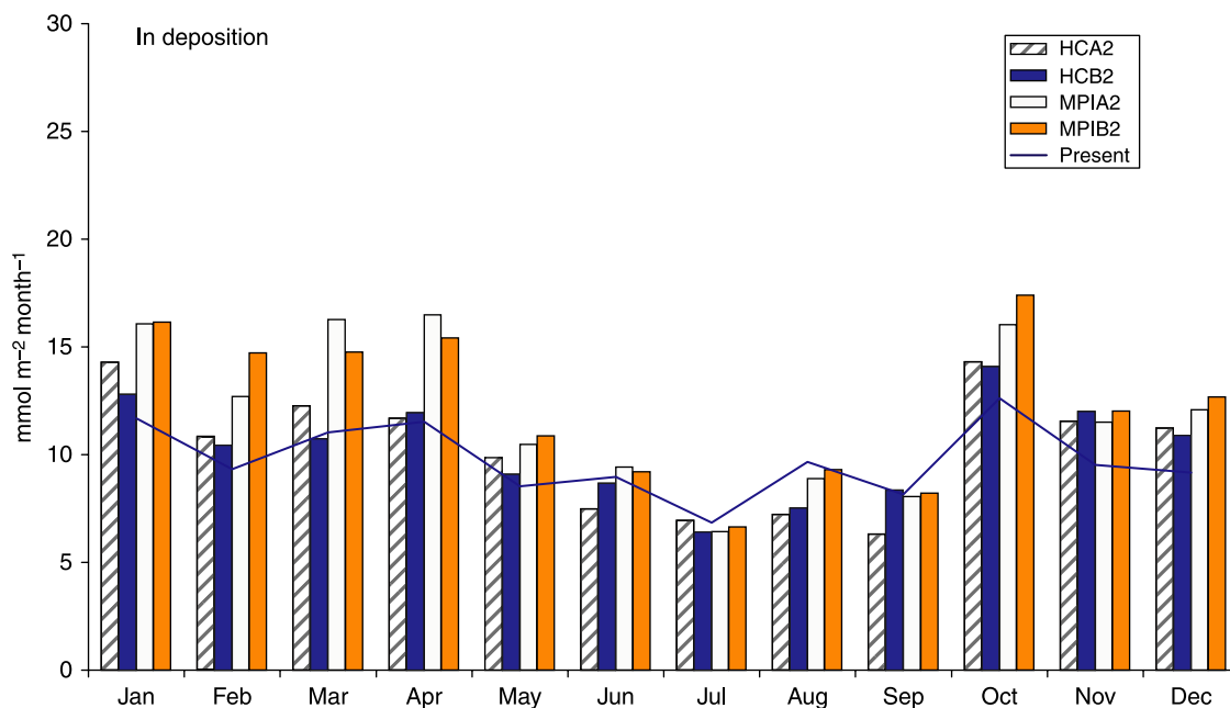
Figure 3 | Monthly present (solid line) mean (1993–2004) and estimated mean (2085–2096) DIN deposition (mmol m -2 month -1 ) for each of the four climate scenarios (bars). Striped, black, white and grey bars represent HCA2, HCB2, MPIA2 and MPIB2 scenarios, respectively.
