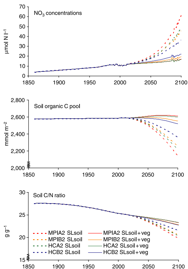
Figure 5 | Simulated mean annual NO 3 surface water concentration, \mu\text{mol l}^{-1} (upper panel), soil organic C pool, \text{mmol m}^{-2} (middle panel) and soil C/N ratio, \text{g g}^{-1} (lower panel) for SLsoil (dashed lines) and SLsoil + veg (solid lines) during 1860–2100. Green, blue, red and orange lines represent HCA2, HCB2, MPIA2 and MPIB2 scenarios, respectively.
