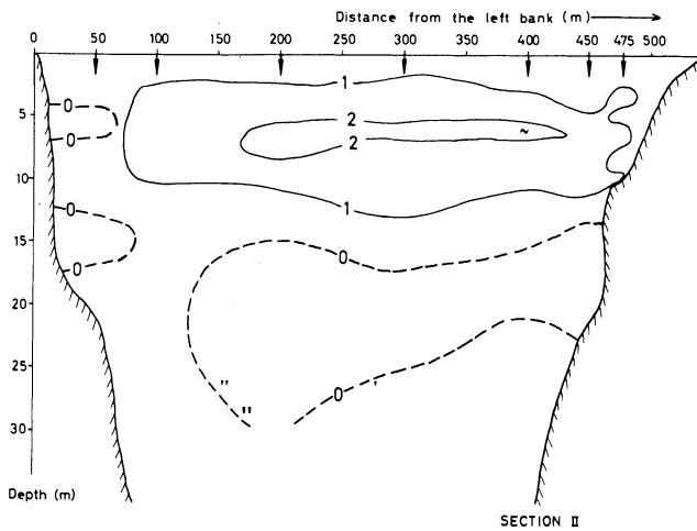
Fig. A4. Velocities in cm/s parallel to the lake axis in the Sperillen, section II on 20/2 1974. The current is directed towards south except in the area bounded by the broken line, where the current is towards north. The location of the measured section II is found in Fig. A1.
