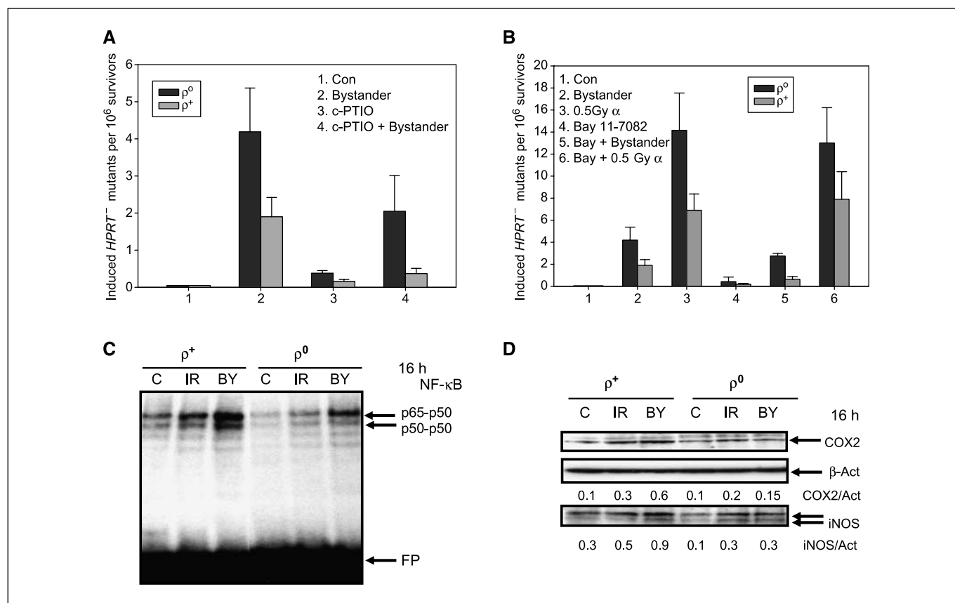
Figure 3. A, effect of the NO scavenger c-PTIO (20 \mu\text{mol/L} , 2 h before and maintained overnight after irradiation) on HPRT^- mutant fractions of \rho^+ and \rho^0 cells. B, effect of the NF- \kappa B inhibitor Bay 11-7082 (1 \mu\text{mol/L} , 2 h before and maintained overnight after irradiation) on HPRT^- mutant fractions of \rho^+ and \rho^0 cells. Data are from three to four independent experiments; bars, SD. C, characterization of NF- \kappa B DNA-binding activities of control, bystander cells, and directly irradiated (0.5 Gy dose of \alpha -particles) \rho^+ and \rho^0 cells using EMSA. FP, free-labeled oligonucleotide probe. D, Western blot analysis of COX-2 and iNOS protein levels in bystander and directly irradiated (0.5 Gy dose of \alpha -particles) \rho^+ and \rho^0 cells. \beta -Actin was used as loading control.
