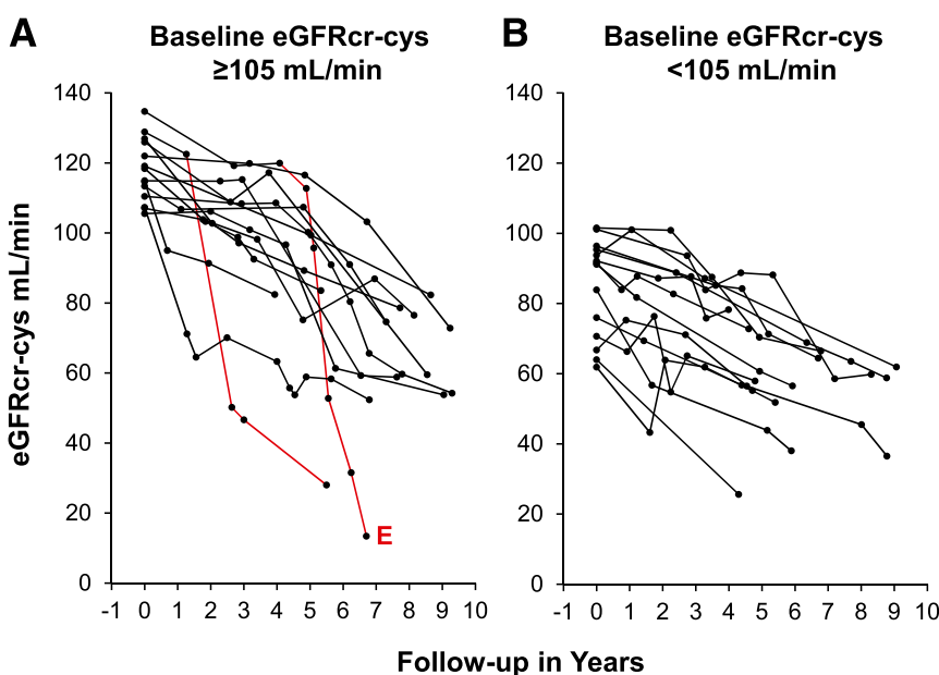
Figure 1 —eGFRcr-cys trajectories in T1D patients with NA and progressive renal decline (loss \geq 3.3% per year) during 4–10 years of follow-up. The trajectories are plotted in patients with baseline eGFRcr-cyst \geq 105 mL/min (A) and in patients with baseline eGFRcr-cys < 105 mL/min (B). Lines in red indicate presence of macroalbuminuria. E, ESRD.
