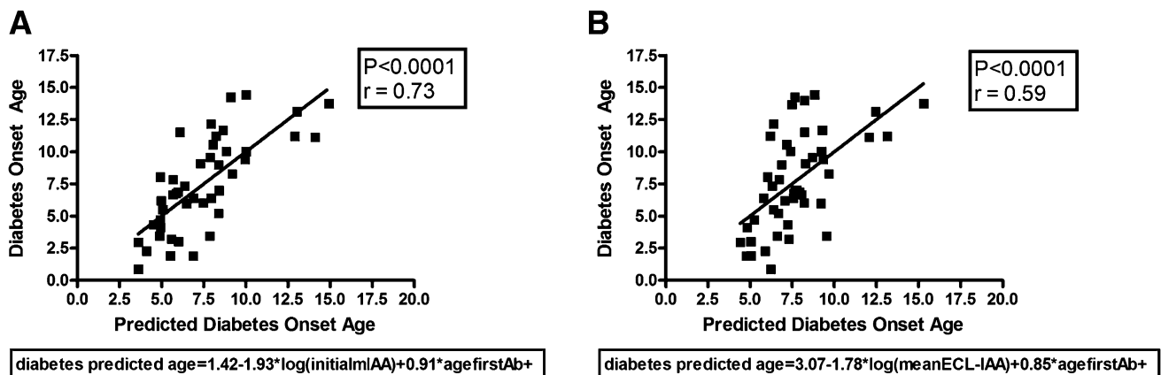
Figure 2 —Predicted age of onset of diabetes. Multiple linear regression was used to evaluate potential predictors of age of diabetes onset, including age at first positive antibody (Ab), initial number of positive antibodies, family history, high-risk HLA-DR3/4, ethnicity, and IAA, GAD, IA-2, and ZnT8 levels (both initial and mean antibody levels). For the first model including initial antibody levels, only initial mIAA levels (loginitialmIAA) and age at first positive antibody (agefirstAb+) were significant predictors of diabetes onset age (A). When analyzing mean antibody levels (B), diabetes onset age was best predicted by mean ECL-IAA levels (logmeanECL-IAA) and age at first positive antibody (agefirstAb+).
