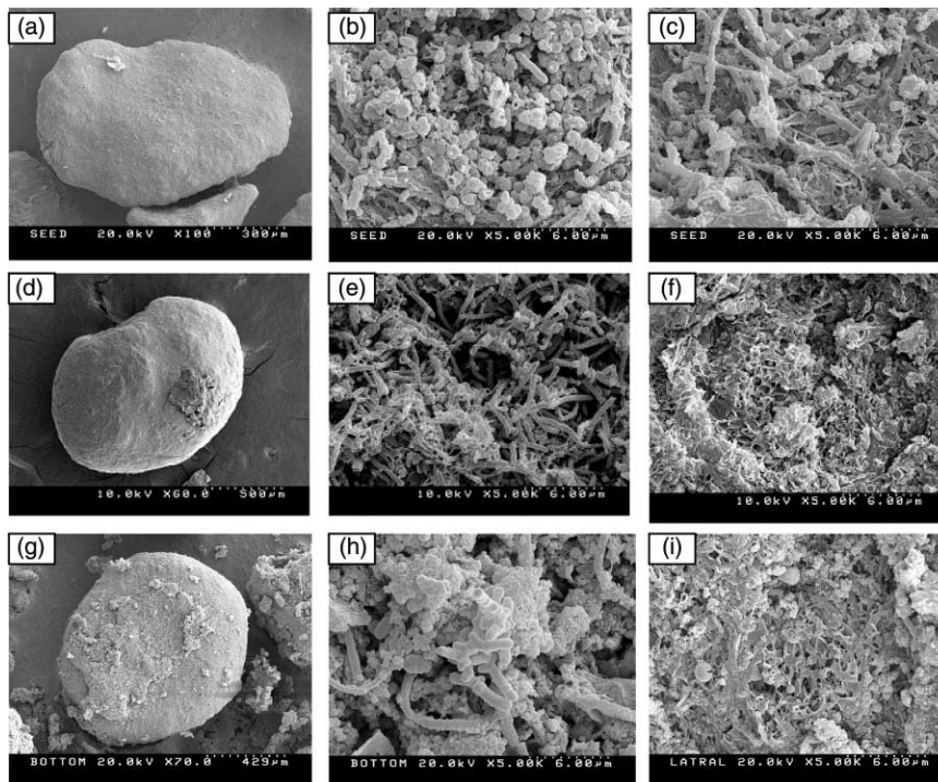
Figure 4 Scanning electron micrographs of granules: (a), (b) & (c), granules at start-up operation; (d), (e) & (f), granules in methanogenic reactor after 5 months; (g), (h) & (i), granules in ANAMMOX reactor after 5 months)
