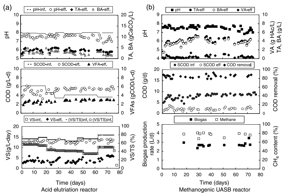
Figure 2 Performance of the ADEPT process
