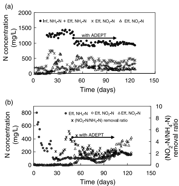
Figure 3 Nitrogen conversion behaviour in SHARON and ANAMMOX reactor
