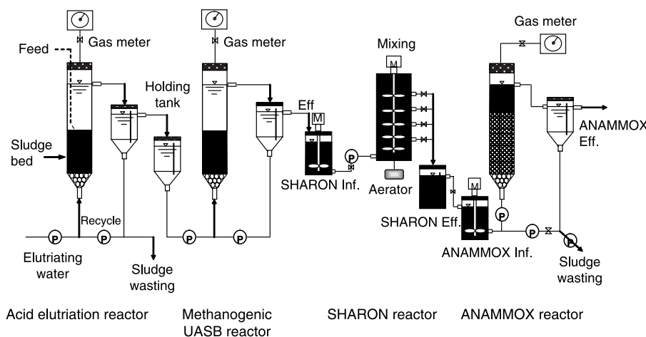
Figure 1 Schematic diagram of sequencing ADEPT and combined SHARON/ANAMMOX processes
