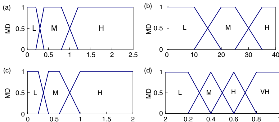
Figure 5 | Membership degree. (a) Water depth, m, (b) water temperature, °C, (c) velocity, m/s, (d) Habitat Suitable Index (HSI). MD = Membership degree, L = Low, M = Medium, H = High and VH = Very high.
