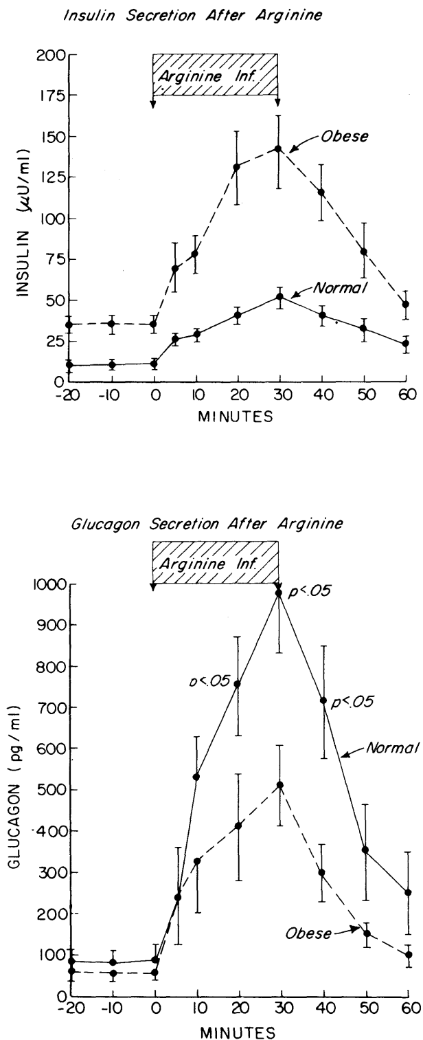
FIG. 2. Effect of arginine infusion on the concentrations of serum insulin (top) and glucagon (lower) in normal weight and obese patients.
