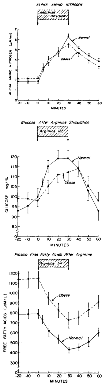
FIG. 1. Effect of arginine infusion on the concentrations of serum alpha amino nitrogen (top), glucose (middle), and free fatty acid (lower) in normal weight and obese patients.
