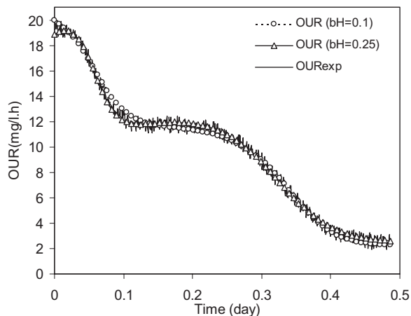
Figure 5 Fitting the OUR profile for domestic sewage for b_H 0.1 and 0.25 d^{-1}
