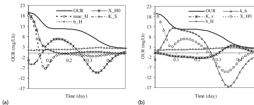
Figure 2 Sensitivity analysis for (a) growth and (b) hydrolysis processes on the OUR curve obtained for domestic sewage [ F/M = 1.35 \text{ gCOD}(\text{g cell COD})^{-1} ]
